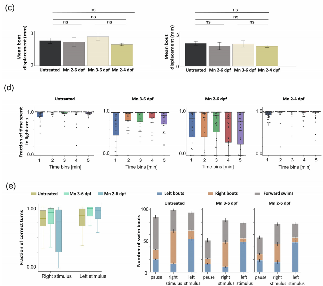
Figure 6. MnCl 2 exposure effects on zebrafish larval behavior during light and dark conditions, as demonstrated by (a) bout number. One-way ANOVA. *** p < 0.001 ; ** p = 0.020 ; (b) mean bout velocity (** p = 0.020 ) and (c) displacement; ns, not significant. Data presented as mean \pm standard error of the mean (SEM); (d) fraction of time spent in the illuminated half field, separated in time bins of 1 min each for untreated, Mn 2–6 dpf, Mn 3–6 dpf and Mn 2–4 dpf treated larvae; (e left) fraction of correct turns for untreated and MnCl 2 exposed larvae (when subjected to left- and right-oriented whole field motion stimuli). Bar heights represent the means across all fish in each group; error bars represent the SEM. Only directional bouts (i.e., left- and rightward swims, without forward swims) were considered for quantification. One-way ANOVA is not significant. (e right) The number of swim bouts during pause intervals and whole field motion stimuli for unexposed and Mn-exposed larvae. Presented as means \pm SEM. Untreated larvae: (a–c) n = 36 ; (d) n = 68 ; (e) n = 71 . Mn 2–6 dpf: (a–d) n = 32 ; (e) n = 52 . Mn 3–6 dpf: (a–d) n = 36 ; (e) n = 55 . Mn 2–4 dpf: (a–d) n = 64 .
