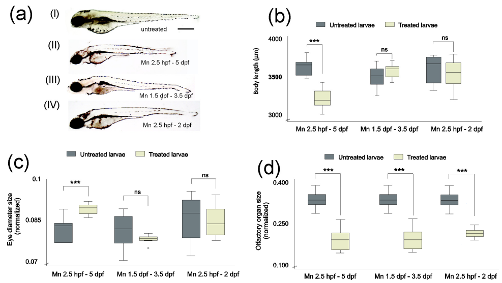
Figure 1. MnCl 2 exposure causes morphological changes in zebrafish larvae at 5 dpf (a(I–IV)), affecting body length (b), eye diameter (c) and olfactory organ size (d). (a(I–IV)) Representative images of zebrafish larvae at 5 dpf unexposed (I) and exposed to 500 µM MnCl 2 at the given durations (II–IV). One-way ANOVA (b,d) *** p < 0.001; (c) *** p = 0.003; ns. not significant, ° correspond to outliers. n = 8 larvae per condition. Scale bar: 100 µm. Data presented as mean ± standard deviation (SD).
