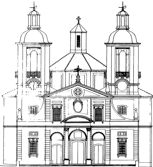
ALZADO PRINCIPAL
