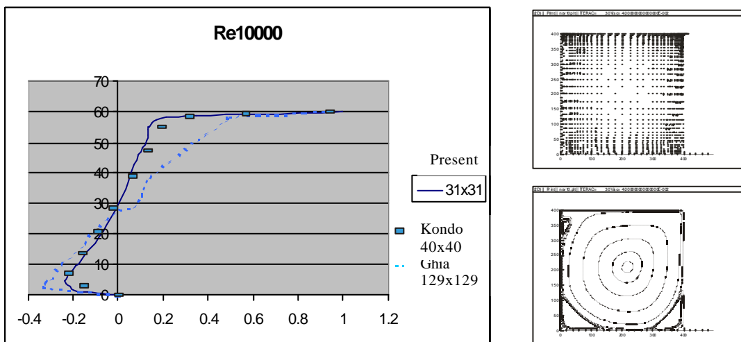
Fig 5.- Horizontal velocities along a central vertical line compared with those of Kondo [4] Ghia [2] for a Reynolds number of 10000. Velocity field and streamlines.
