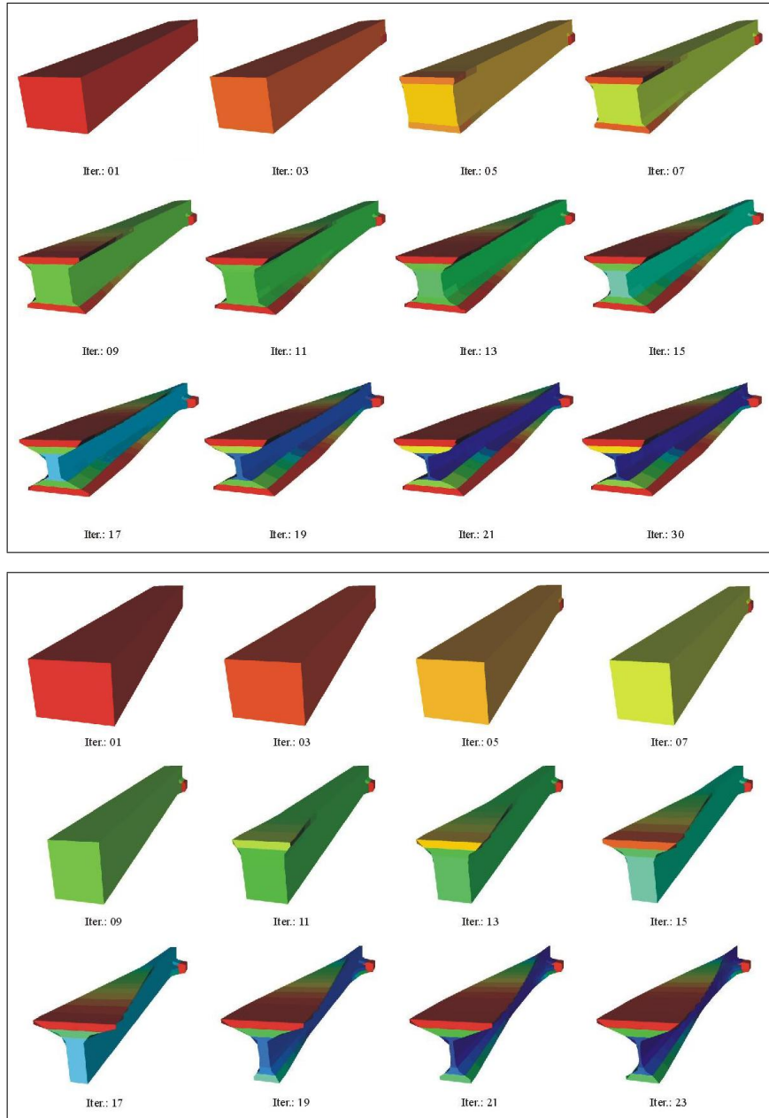
Figure 2: MWSC topology optimization of a simply supported structure, with small height/length ratio, considering sliding (up) and fixed (down) supports. Concentrated load applied in the center of the upper side. (Note: only half of the solid is represented in order to show the central section.)
