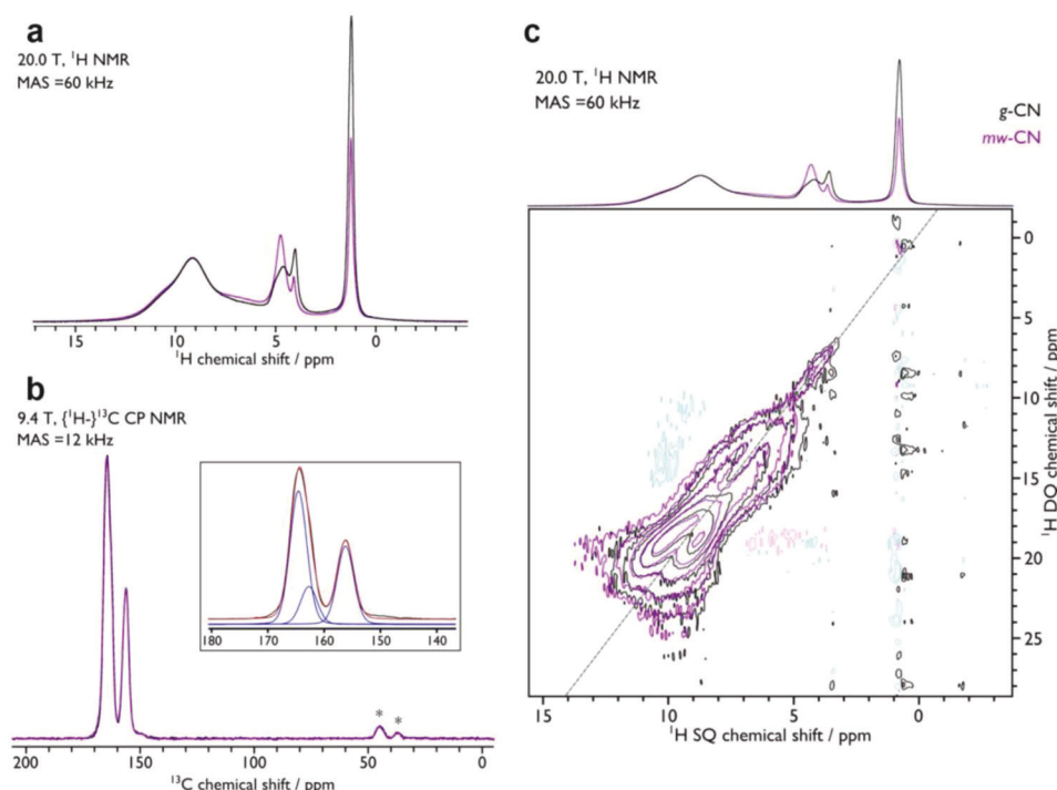
Figure 2. a) ^1\text{H} Hahn-echo MAS NMR spectra of g -CN (black) and mw -CN (purple), recorded at 20.0 T using a MAS frequency of 60 kHz at ambient temperature. b) \{^1\text{H}\}\text{-}^{13}\text{C} CPMAS NMR spectra of g -CN (black) and mw -CN (purple), recorded at 9.4 T using a MAS frequency of 12 kHz at ambient temperature. The inset shows the peak deconvolution. c) 2D ^1\text{H} MAS NMR homonuclear Double quantum–single quantum (DQ–SQ) dipolar correlation spectra of g -CN (black) and mw -CN (purple), recorded at 20.0 T using the S_2 recoupling sequence and a MAS frequency of 60 kHz at ambient temperature. The dashed line highlights the DQ diagonal and the corresponding 1D spectra are reproduced from (a) above for comparison. The 2D DQ–SQ spectrum in (c) aids the assignment of the ^1\text{H} resonances, which are consistent with those for similar polymeric carbon nitride. [24a] The absence of a correlation peak with the resonance at \delta\{^1\text{H SQ}\} = 1.3 ppm indicates that this must correspond to discrete protons that are >2 Å from another and as such corresponds to lone H on bridging N ( -\text{NH}- ). The autocorrelation peaks at \delta\{^1\text{H SQ}\} = 4\text{--}5 ppm, which lack cross-correlation peaks, correspond to nonhydrogen-bonded \text{NH}_2 groups. The correlation peaks at \delta\{^1\text{H SQ}\} = 6\text{--}8 ppm correspond to H on bridging N that are in proximity to other protons, possibly indicating weak H-bonding, while those at \delta\{^1\text{H SQ}\} = 8\text{--}11 ppm correspond to protons involved in strong H-bonding, either from \text{NH}_2 or H on bridging N.
