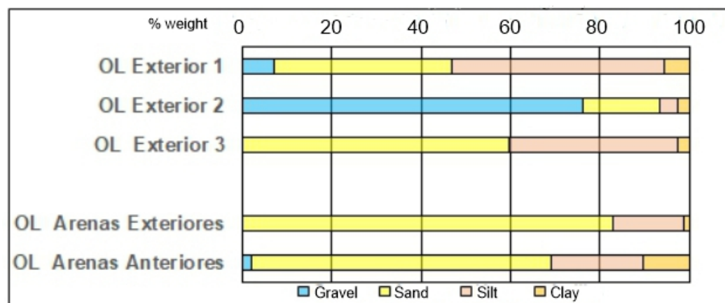
Figure 11. El Olivo Cave, outer excavation and samples of sand; granulometry of the total fraction.
