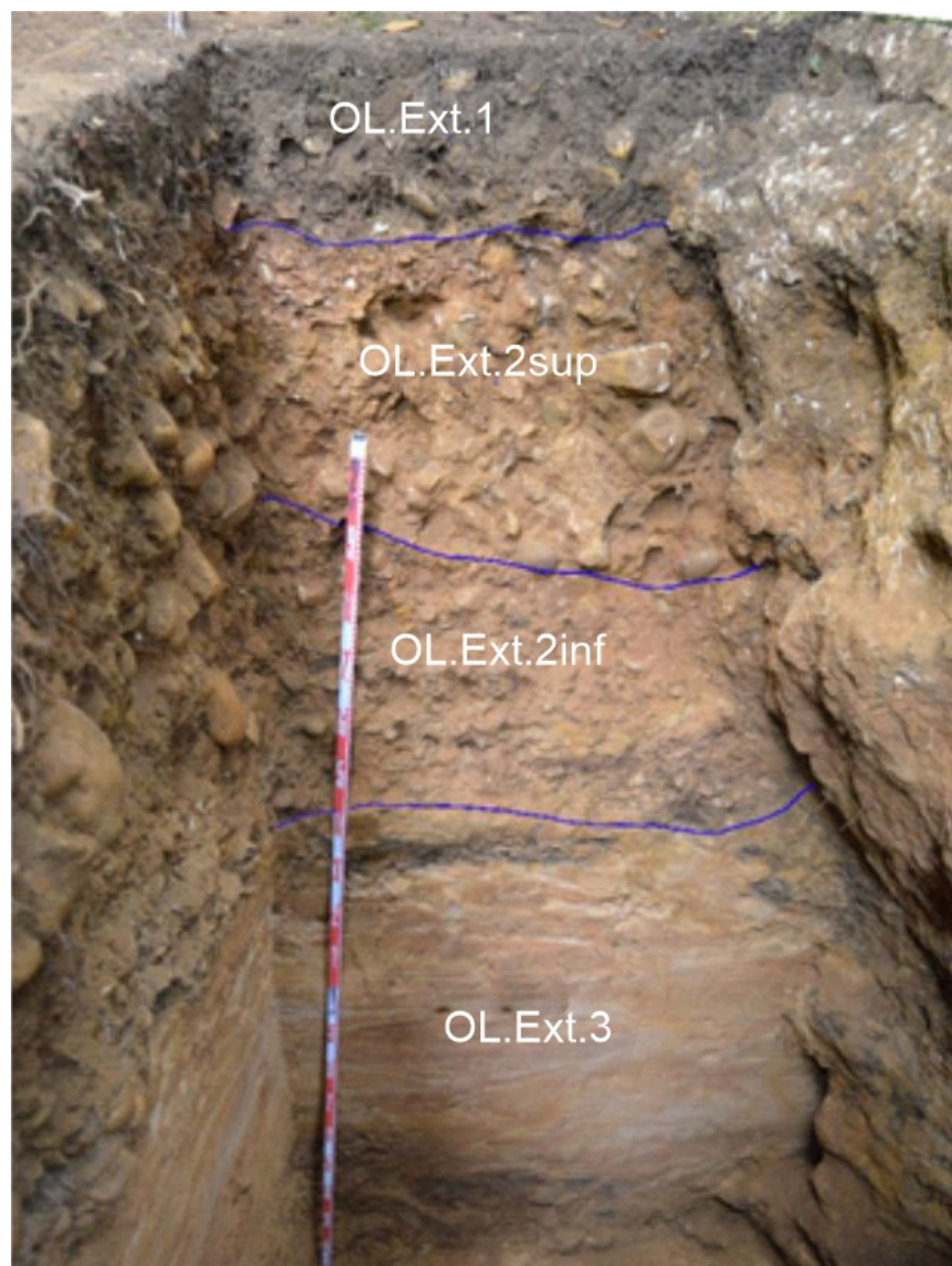
Figure 9. El Olivo Cave. Stratigraphy outside the cave (the scale is 2 m).
