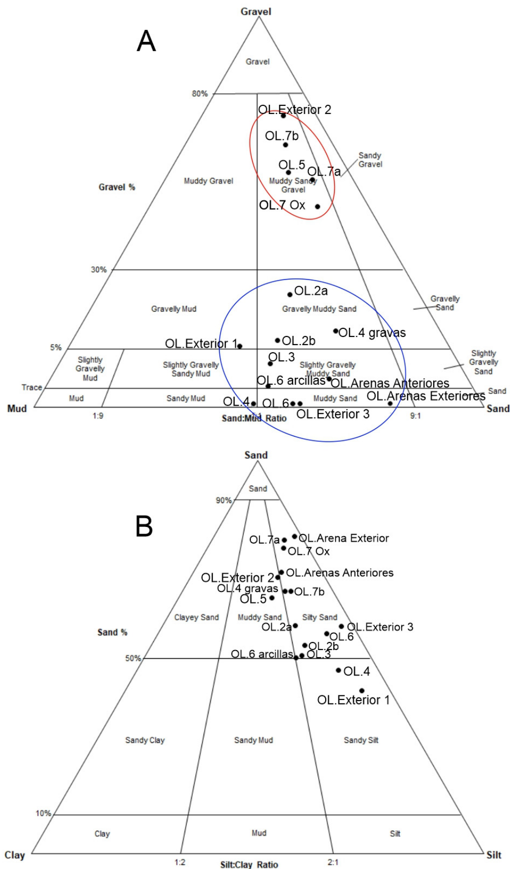
Figure 12. El Olivo Cave. (A) A triangular diagram representing the total fraction of the sediments from the interior and exterior excavations. (B) A triangular diagram representing the fine fraction (<2 mm) of sediments from the interior and exterior excavations.
