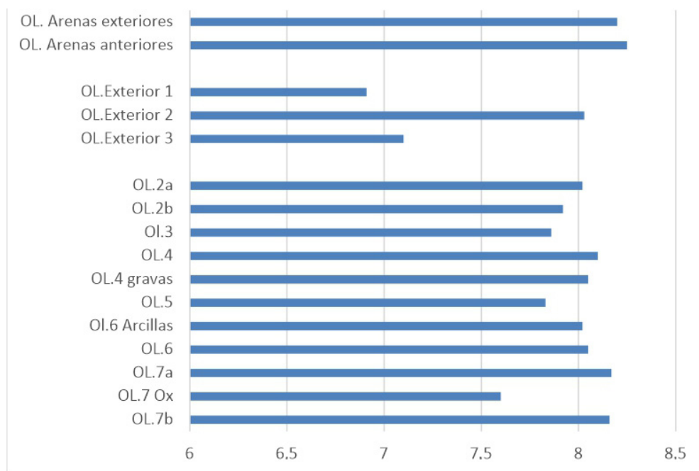
Figure 16. El Olivo Cave. pH of the sediments from the interior and exterior excavations.
