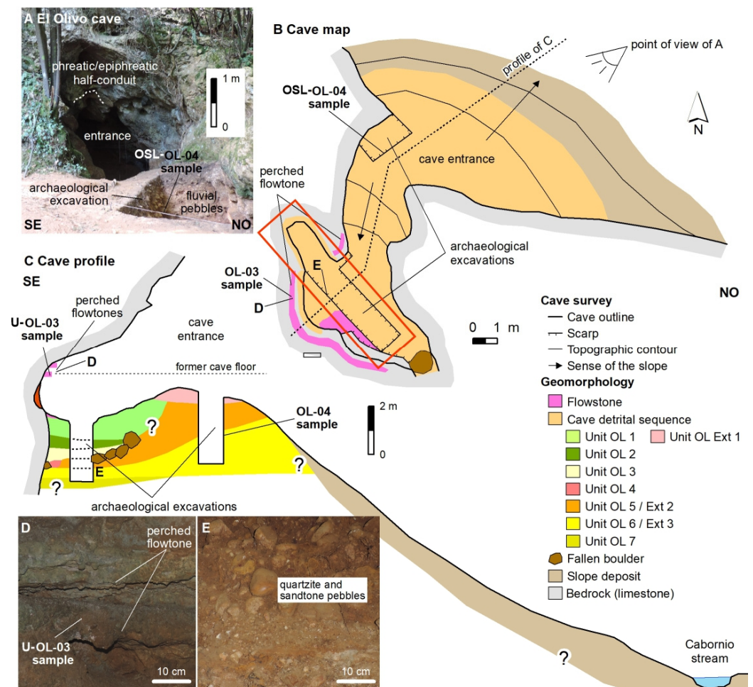
Figure 4. (A) El Olivo Cave showing the archaeological excavation into fluvial deposits at the cave entrance. (B) The cave geomorphological map with the perched flowstone projected outside the cave outline is preserved on the cave walls. (C) Profile from the cave to the present-day fluvial network, showing the position of the perched flowstone (which marks a former cave floor) and the cave detrital
