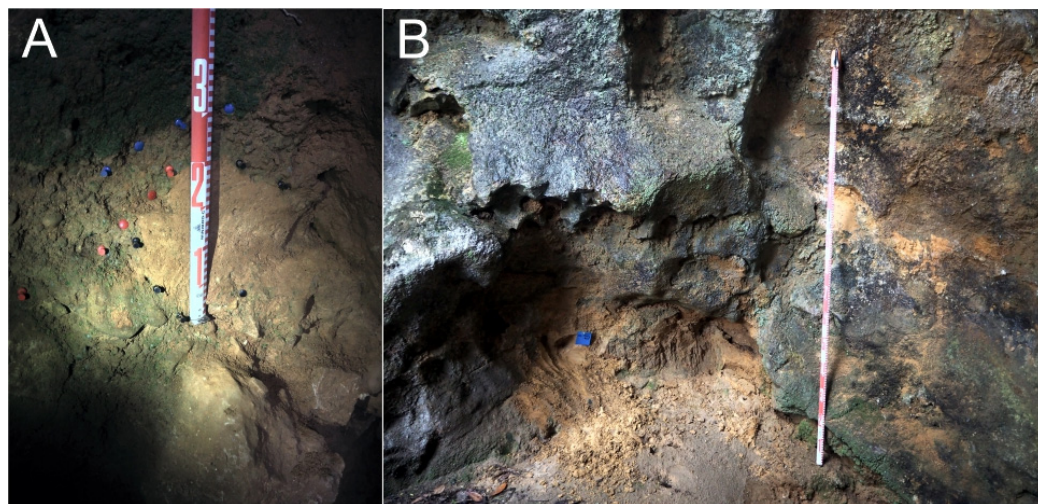
Figure 8. El Olivo Cave. Photographs of the sampling points of OL.Arenas anteriores (A) and OL.Arenas exteriores (B).
