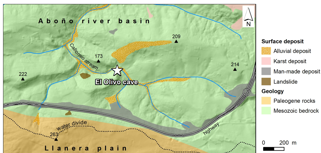
Figure 5. Alluvial deposits associated with the Cabornio stream in the surroundings of El Olivo Cave. Alluvial sediments came from the erosion of the Llanera plain, made of Paleogene conglomerate and sandstone. The plain surface is being captured by the Aboño River basin at the present time. The star indicates the location of the El Olivo Cave. Numbers indicate the altitudes above sea level in m of the main elevations.
