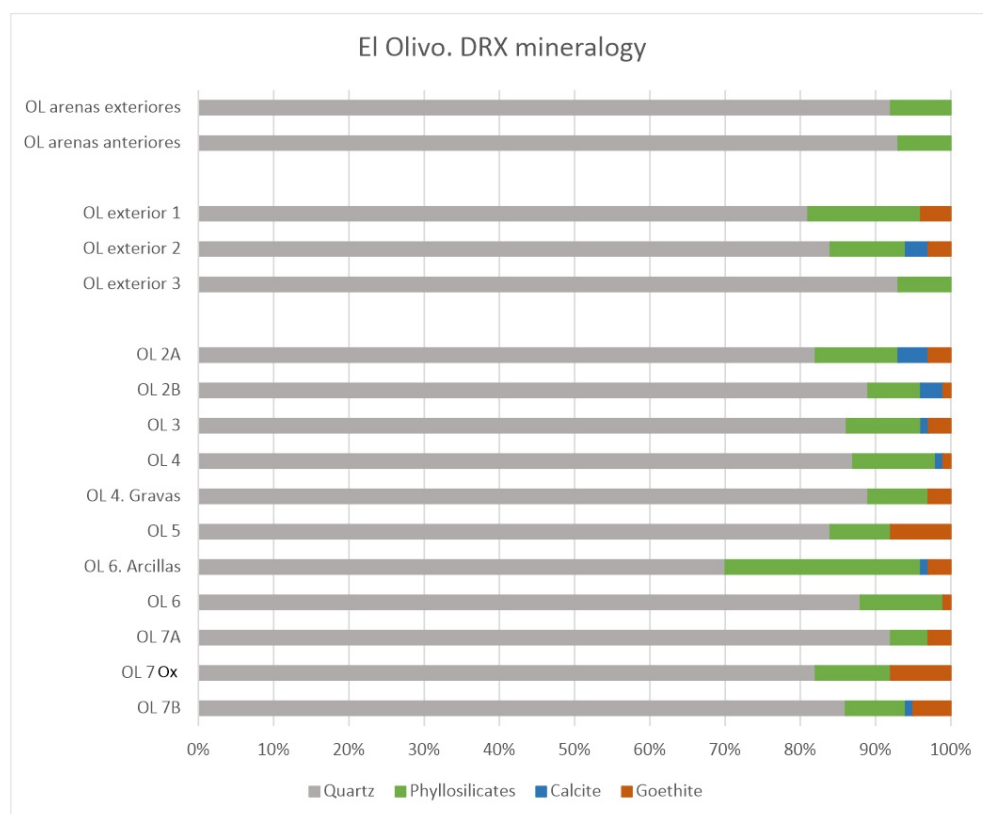
Figure 14. El Olivo Cave. XRD mineralogy of the fine fraction of the sediments from the interior and exterior excavations.
