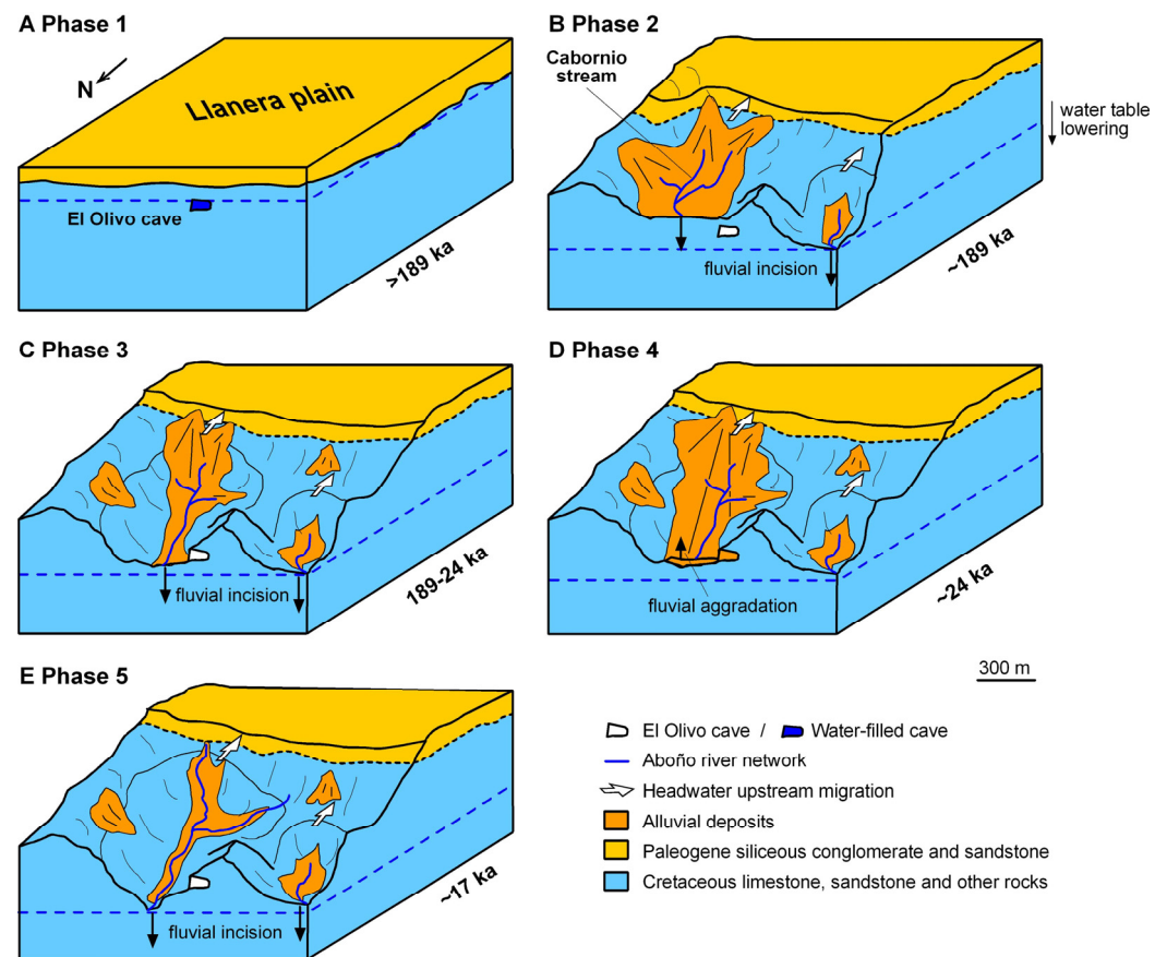
Figure 17. Paleogeographic evolution of El Olivo Cave: (A) Phase 1: Cave formation within Cretaceous bedrock covered by Paleogene rocks (Llanera plain). (B) Phase 2: Erosion of the northern Llanera plain due to fluvial incision and headwater upstream migration; cave aggradation until 189 \pm 17 ka. (C) Phase 3: Partial erosion of the former cave infill coeval to fluvial incision. (D) Phase 4: Alluvial deposition inside the cave in relation to alluvial fans during OIS-2. (E) Phase 5: Fluvial incision up to present-day coevally with human frequentation. The blue dashed lines indicate the water table.
