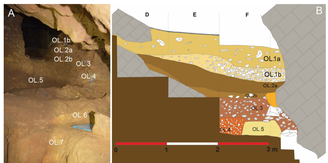
Figure 7. El Olivo Cave. Interior trench stratigraphy: (A) photography and (B) stratigraphic section. In (B), capital letters D, E and F correspond to the name of the squares of the excavation.
