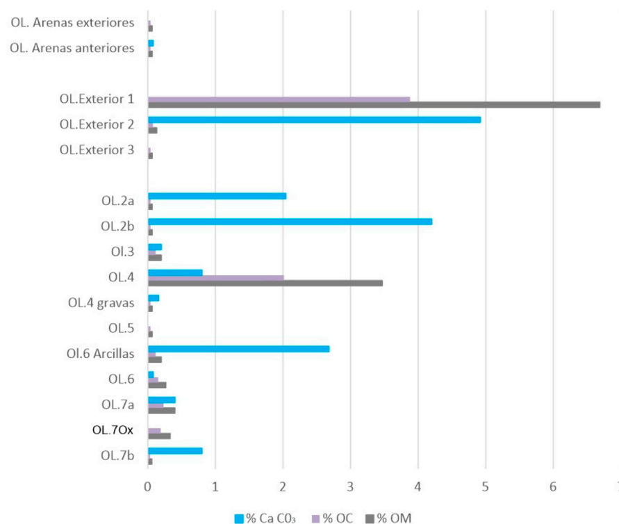
Figure 15. El Olivo Cave. Calcium carbonate, organic carbon, and organic matter of the sediments from the interior and exterior excavations.
