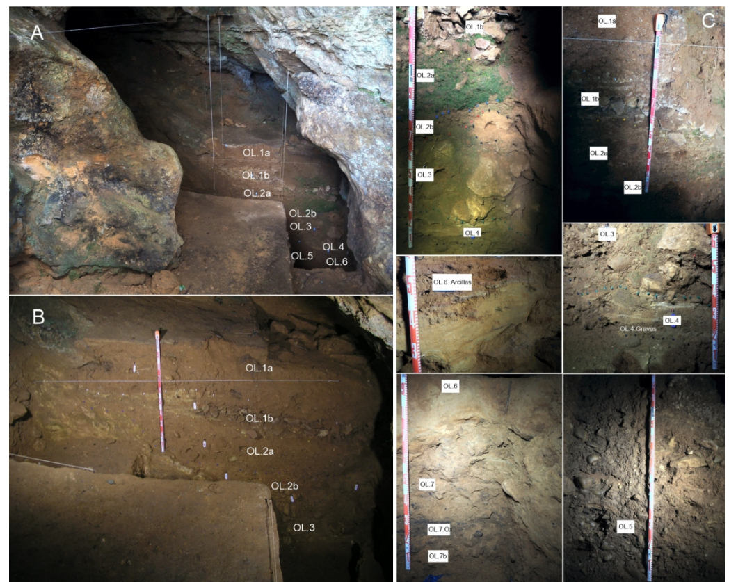
Figure 6. El Olivo Cave. (A) General view of the stratigraphic profile from the entrance. (B) Detail of the previous view. (C) Details of the stratigraphic sequence.
