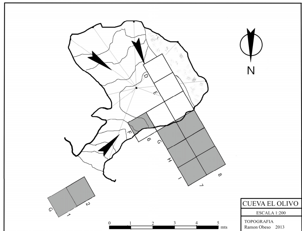
Figure 3. El Olivo Cave plan [4], with indication of the excavation grid and the excavated squares (in gray) (numbers and capital letters indicate the names of the excavated squares; black arrows indicate slopes).
