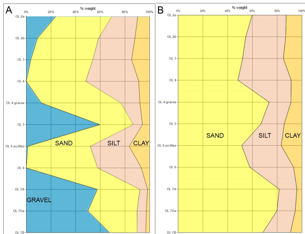
Figure 10. El Olivo Cave, inner excavation. (A) Granulometry of the total fraction. (B) Granulometry of the fine fraction (<2 mm).
