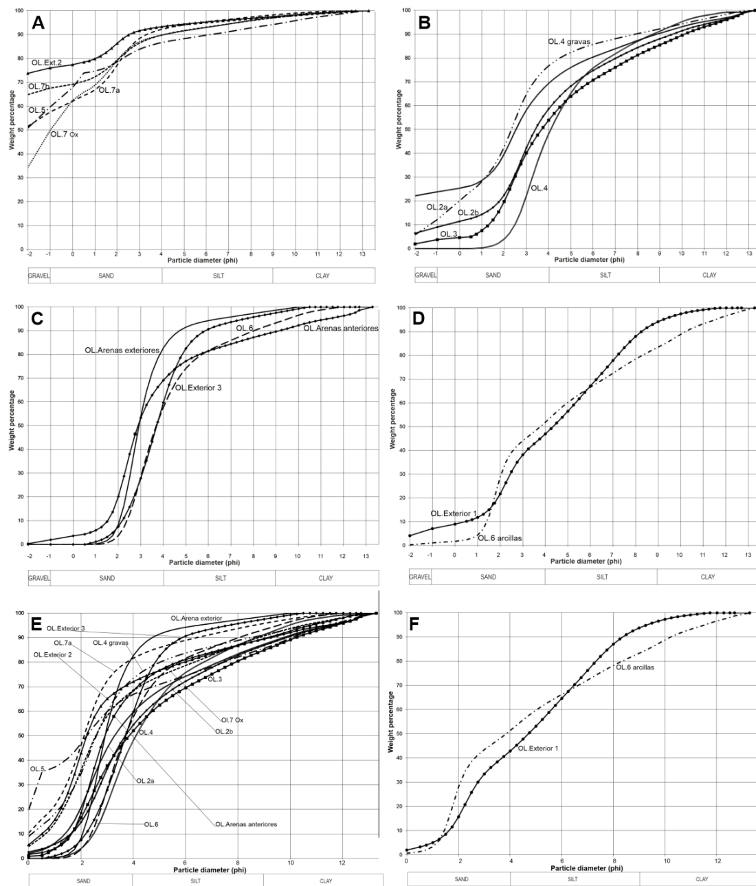
Figure 13. El Olivo Cave. Granulometric curves representing the total fraction of the samples of G-A (A), G-B1 (B), G-B2 (C), and G-B3 (D) families, and the fine fraction of the samples of F-1 (E) and F-2 (F) families.
