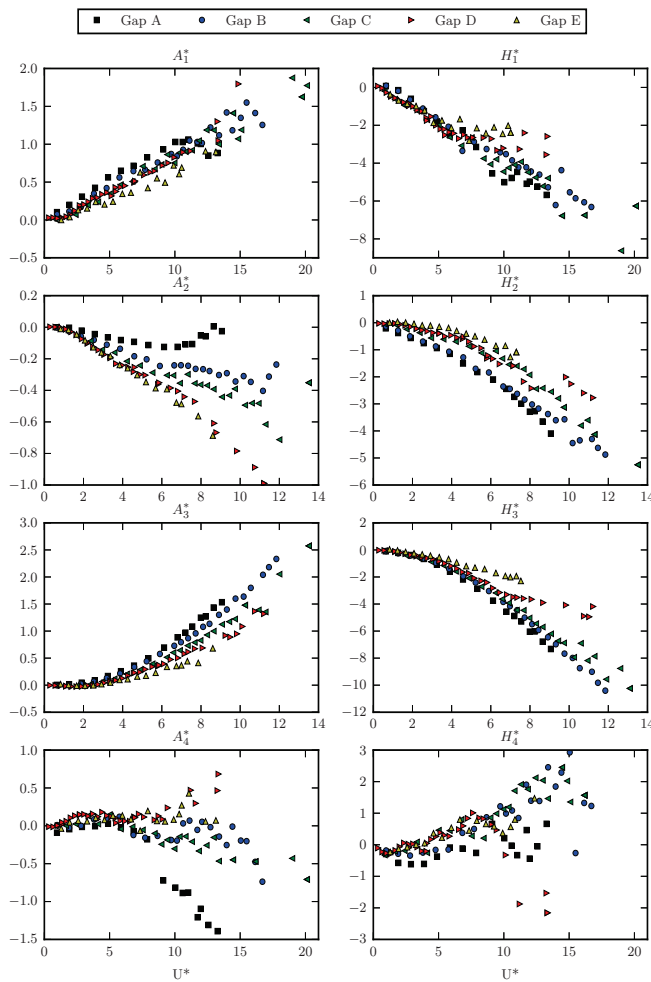
Figure 6: Flutter derivatives for Gaps A, B, C, D and E.
