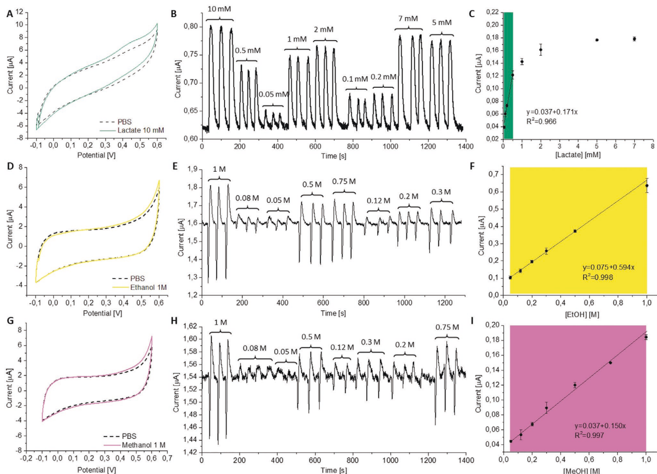
Figure 5. Electrochemical responses of inks produced with LOx and AOx. A) CV responses of EEG-LOx-CoPC inks deposited over C-SPE in PBS, in the absence and in the presence of 10 \times 10^{-3} M lactate (scan rate 20 \text{ mV s}^{-1} ). B) Representative FIA response of EEG-LOx-CoPC ink deposited on C-SPE. Nine different lactate concentrations were tested, namely, 0.05 \times 10^{-3} , 0.1 \times 10^{-3} , 0.2 \times 10^{-3} , 0.5 \times 10^{-3} , 1.0 \times 10^{-3} , 2.0 \times 10^{-3} , 5.0 \times 10^{-3} , 7.0 \times 10^{-3} , and 10.0 \times 10^{-3} M, in a randomized manner. C) Plot of the current intensities registered in FIA versus lactate concentration. The highlighted linear regime spans between 0.05 \times 10^{-3} and 5.0 \times 10^{-3} M. Error bars represent the standard deviation among three injections in the same analysis. D) CV responses of EEG-AOx-CoPC ink deposited over C-SPE in PBS, in the absence and in the presence of 1.0 \text{ M} EtOH (scan rate 20 \text{ mV s}^{-1} ). E) Representative FIA response of EEG-AOx-CoPC ink deposited on C-SPE. Eight different EtOH concentrations were tested, namely, 0.05, 0.08, 0.12, 0.2, 0.3, 0.5, 0.75, and 1.0 \text{ M} , in a randomized manner. F) Plot of the current intensities registered in FIA versus EtOH concentration. The highlighted linear regime spans between 0.05 and 1.0 \text{ M} . Error bars represent the standard deviation among three injections in the same analysis. G) CV responses of EEG-AOx-CoPC ink deposited over a C-SPE in PBS, in the absence and in the presence of 1.0 \text{ M} MeOH in PBS (scan rate 20 \text{ mV s}^{-1} ). H) Representative FIA of EEG-AOx-CoPC ink deposited on C-SPE. Eight different MeOH concentrations were tested, namely, 0.05, 0.08, 0.12, 0.2, 0.3, 0.5, 0.75, and 1.0 \text{ M} , in a randomized manner. I) Plot of the current intensities registered in FIA versus MeOH concentration. The highlighted linear regime spans between 0.05 and 1.0 \text{ M} . Error bars represent the standard deviation among three injections in the same analysis.
