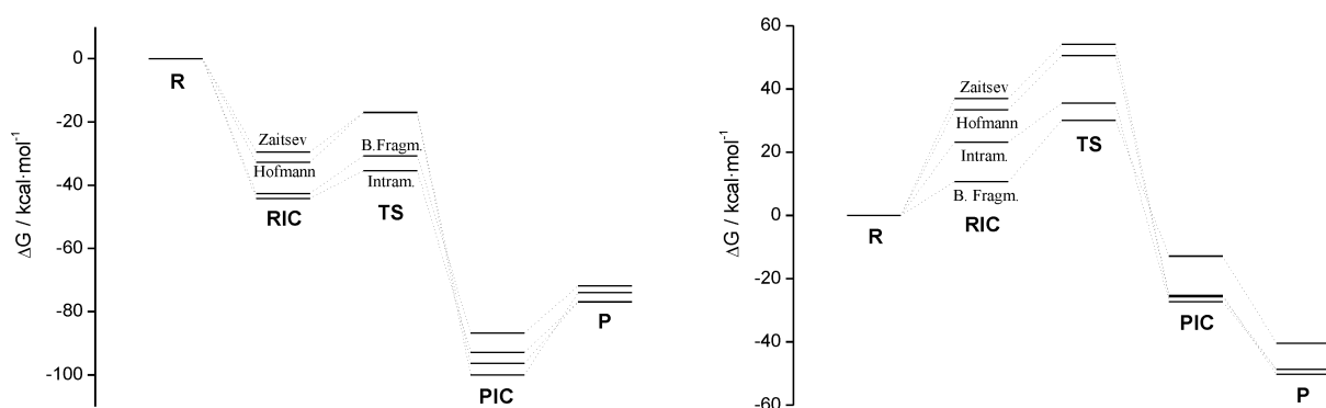
Fig. 1 Gibbs free energy profiles for the four pathways found for the HO - -promoted decomposition of N -chloro, N -methylethanolamine at the MP2=full/6-31++G(d,p) computational level. Reactants (R) were taken as reference. Data obtained with microsolvated (left) and microsolvated plus continuum (right) models.
