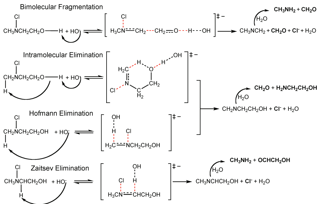
Scheme 2 The four parallel pathways involved in the rate-determining step of the HO - -promoted decomposition of N -chloro, N -methylethanolamine. Bonds being broken (in red) and formed (in black) are shown as dashed lines. End products through each pathway are shown in bold. Notice that the products of Hofmann and intramolecular eliminations are the same, and thus these two pathways are indistinguishable by product analysis.
