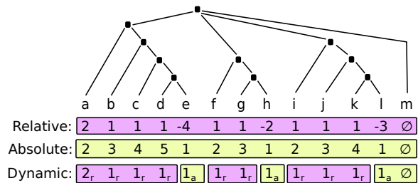
Figure 4: A synthetic constituent tree where n_t is encoded using a relative scheme, a top-down absolute scale, and an ideal dynamic combination. The relative scheme is appropriate to open and close short constituents, but becomes sparse when encoding the large ones, e.g. n_t for the tokens ‘e’, ‘h’ and ‘l’. The opposite problem is observed for the top-down absolute scheme (e.g. tokens from ‘a’ to ‘d’). The dynamic linearization combines the best of both encodings (we use the subscript ‘r’ to denote the labels coming from the relative encoding, and ‘a’ from the absolute one).
