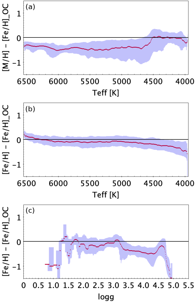
Fig. 11. Difference between GSP-Phot metallicities of individual FGK members and the mean [\text{Fe}/\text{H}] of the parent open cluster for stars with \frac{\sigma_{\text{par}}}{\sigma_{\text{mag}}} \geq 10 and MARCS models, before and after the calibration. We note that the calibration on LAMOST [\text{Fe}/\text{H}] values translates [\text{M}/\text{H}] to [\text{Fe}/\text{H}] . The red line is the median of the distribution. The blue area is delimited by the 16th and 84th quantiles. Panel (a) : residuals versus T_{\text{eff}} before the calibration. Panel (b) : residuals versus T_{\text{eff}} after the calibration. Panel (c) : residuals versus \log g after the calibration.
