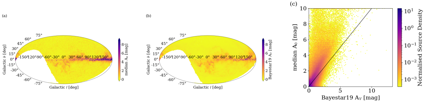
Fig. 14. Extinction comparison between GSP-Phot and Bayestar19 for a randomly selected sample of 1 million sources. Panel (a) : skymap of A_0 provided by GSP-Phot, taking a pixel-wise median value. Panel (b) : skymap of A_V provided by Bayestar19, taking a pixel-wise median value. Panel (c) : one-to-one comparison of the GSP-Phot median A_0 and the Bayestar19 A_V . Both skymaps use the Mollweide projection where lines of constant latitude are horizontal straight lines parallel to the equator. All panels show the identical sample of stars. The missing data in panels (a) and (b) are due to the footprint of Bayestar19.
