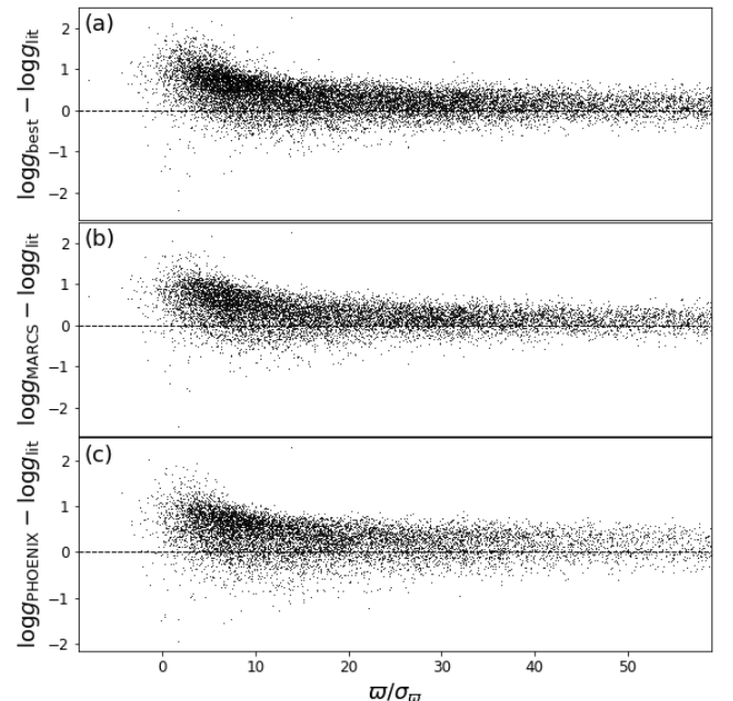
Fig. 9. Bias of surface gravity estimates for stars with low parallax signal-to-noise ratio, \varpi/\sigma_{\varpi} , for 25 169 red clump stars (Jönsson et al. 2020; Bovy et al. 2014). Panel (a): GSP-Phot best-library results. Panel (b): GSP-Phot MARCS library results. Panel (c): GSP-Phot PHOENIX library results.
