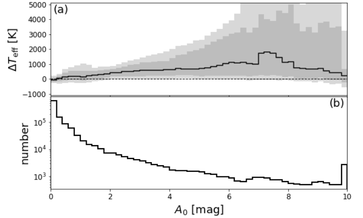
Fig. 7. Impact of extinction onto differences in T_{\text{eff}} between results and literature values. Panel (a) : differences in T_{\text{eff}} between our GSP-Phot results and literature values as function of estimated extinction A_0 for the joint samples from APOGEE DR16 (Jönsson et al. 2020), GALAH DR3 (Buder et al. 2021), LAMOST DR4 (Wu et al. 2011, 2014), and RAVE DR6 (Steinmetz et al. 2020). If the same star appears in more than one literature resource, it enters this plot multiple times with identical GSP-Phot results but different literature values. The data are binned into A_0 ranges of 0.2 mag, where the solid black line indicates the median residual and the two shaded regions show the 5th-to-95th percentiles and the 16th-to-84th percentiles, respectively. Panel (b) : distribution of A_0 estimates in this sample.
