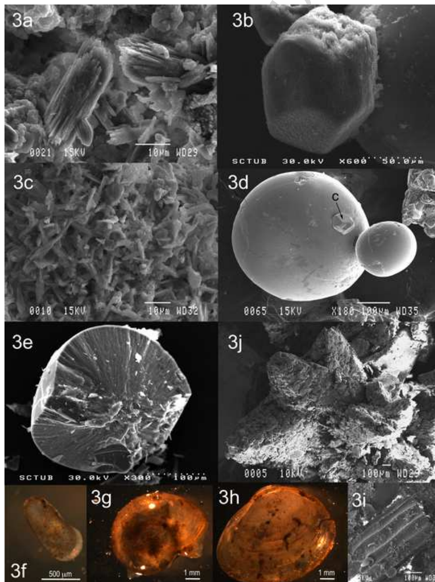
Fig. 3. Carbonate components in the Lake Chungará sediments: 3a) Fibre-bundle calcite crystals. 3b) Subhedral fibre-bundle calcite crystal. 3c) Needle-shaped aragonite crystals. 3d) Aragonite spheroids. Aragonite spheroids coexist with calcite crystals (c). 3e) Inner fibrous-radiated structure of an aragonite spheroid. Ostracoda valves ( Limnocythere sp; 3f), gastropoda ( Biomphalaria ; 3g) and bivalvia ( Pisidium ; 3h) shells and charophyta ( Chara ; 3i) stems and gyrogonites are the main bioclasts in Lake Chungará sediments. 3j) Calcite pseudomorphs (after ikaite?) in core 14.
