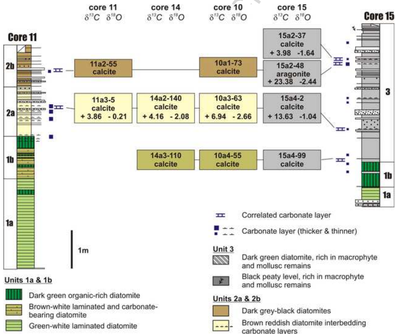
Fig. 4. Some carbonate layers in cores 10, 11, 14 and 15, placed at distances of several kilometres, are correlated. Lateral changes in carbonate mineralogy and in isotopic compositions ( \delta^{13}\text{C}_{\text{VPDB}} , \delta^{18}\text{O}_{\text{VPDB}} ) are reported. Lithologic and stratigraphic units of 11 and 15 cores are included. Name, mineralogy and isotopic compositions for each sample are shown. Samples 15a2-48 and 15a4-2 (in core 15) showing very high \delta^{13}\text{C}_{\text{VPDB}} values reflect methanogenic fermentation.
