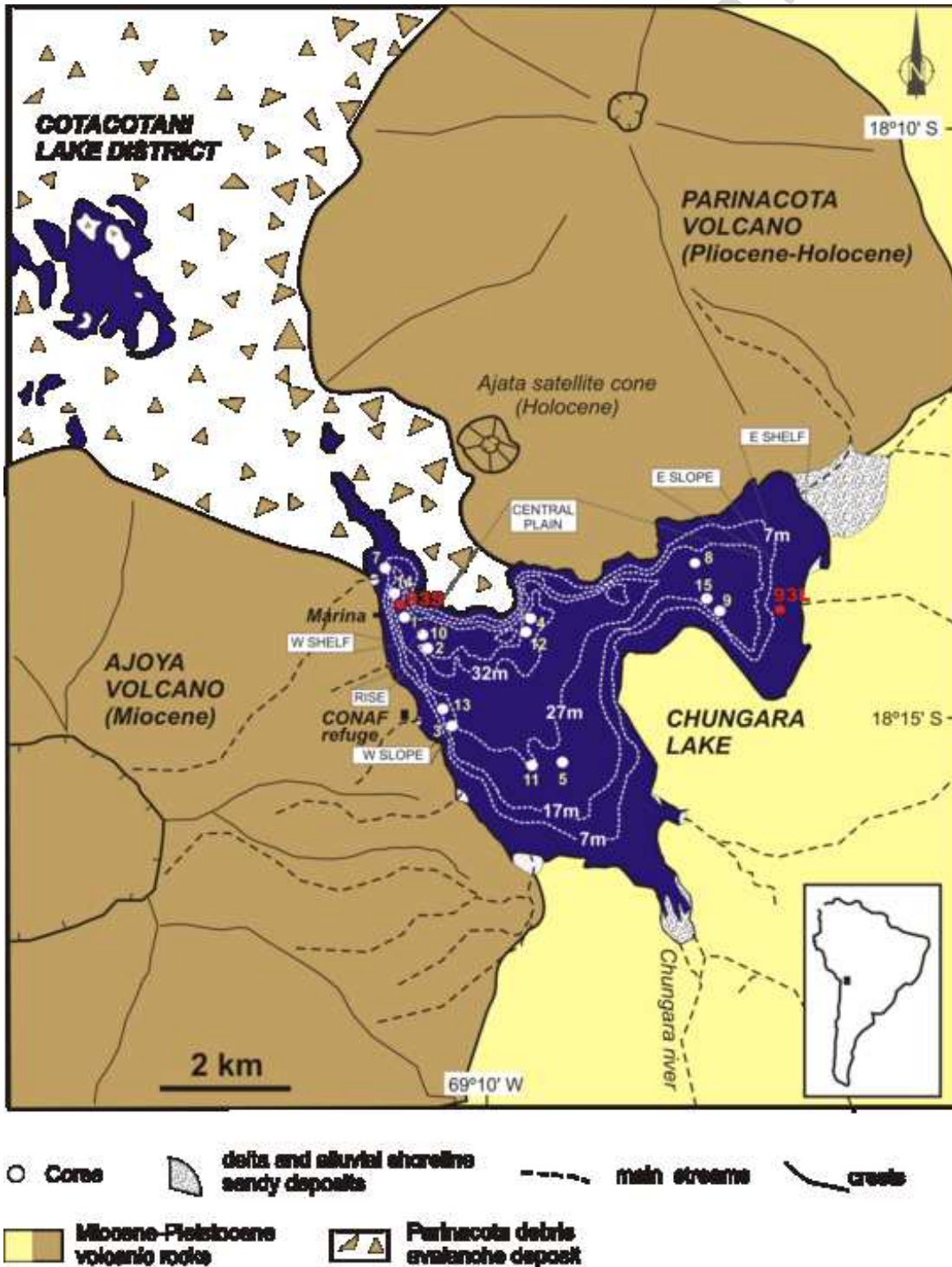
Fig. 1. Geological sketch of the Lake Chungará. Neighbouring volcanoes Ajoya and Parinacota, the Chungará River and the Cotacotani Lake district are included. Sites of all cores and the lake-bottom topography and morphology are also indicated.
