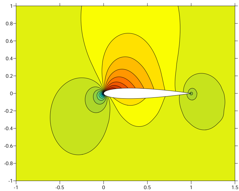
Fig. 14 Subsonic Inviscid flow around a NACA 0012. Mach field and contours.
