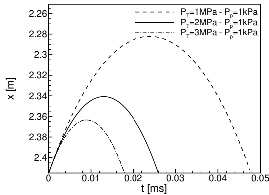
Fig. 9 Numerical solution for deaerated water for different P_T values
