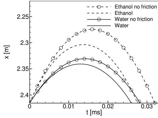
Fig. 6 Numerical solution to equation 6 solved with and without friction for both deaerated water and deaerated ethanol
