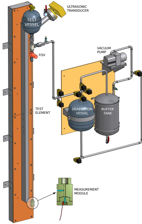
Fig. 1 Experimental facility layout
