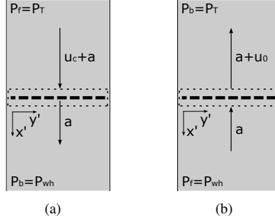
Fig. 5 Control volume used to solve the compression wave (a) and the expansion wave (b) traveling in the liquid column
