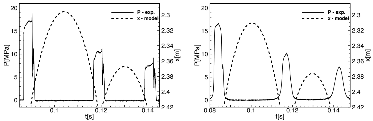
Fig. 11 Theoretical column separation computed for the first and second peak and compared to experimental data. Test case: deaerated ethanol, P_T = 2 \text{ MPa} and P_p = 1 \text{ kPa} (left) and P_p = 10 \text{ kPa} (right)
