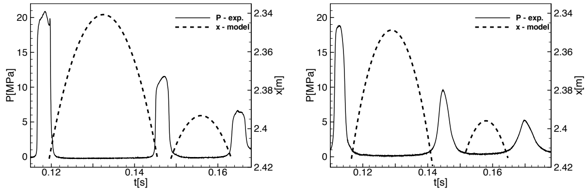
Fig. 10 Theoretical column separation computed for the first and second peak and compared to experimental data. Test case: deaerated water, P_T = 2 \text{ MPa} and P_p = 1 \text{ kPa} (left) and P_p = 10 \text{ kPa} (right)
