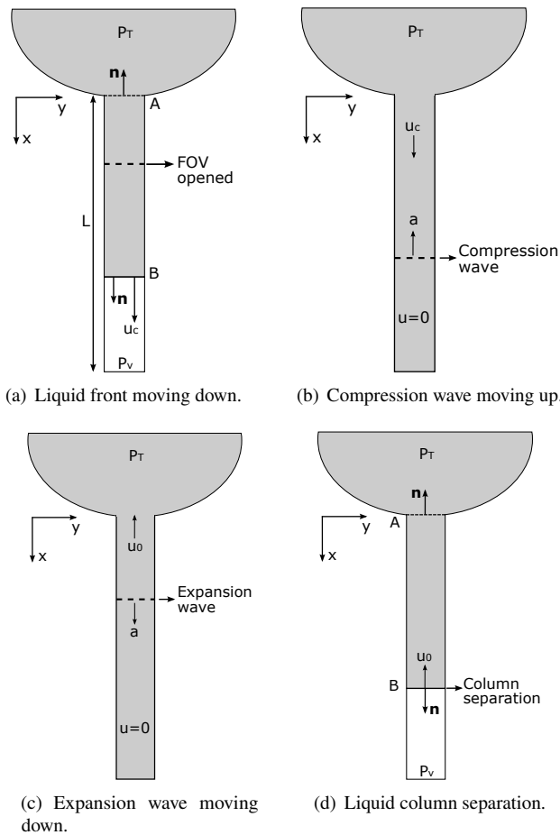
Fig. 4 Sequence of liquid column dynamics.
