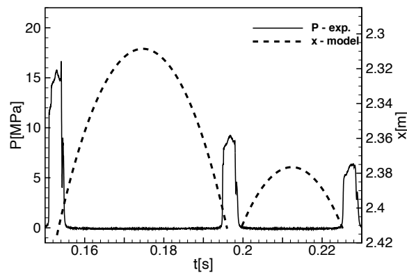
Fig. 12 Theoretical column separation computed for the first and second peak and compared to experimental data. Test case: deaerated water, P_T = 1 \text{ MPa} and P_p = 1 \text{ kPa}
