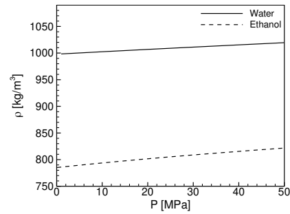
Fig. 3 Density of water and ethanol as a function of pressure. According to Tait's equation
