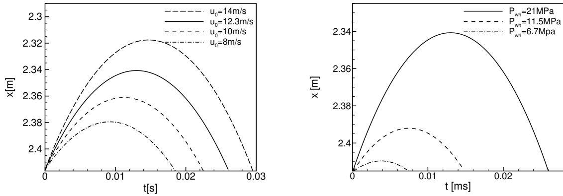
Fig. 7 Comparison of the liquid column separation for different initial velocities with deaerated water Fig. 8 Numerical solution for deaerated water with P_T = 2 \text{ MPa} and different P_{wh} values
