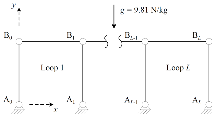
Figure 7: L -loop fourbar linkage
