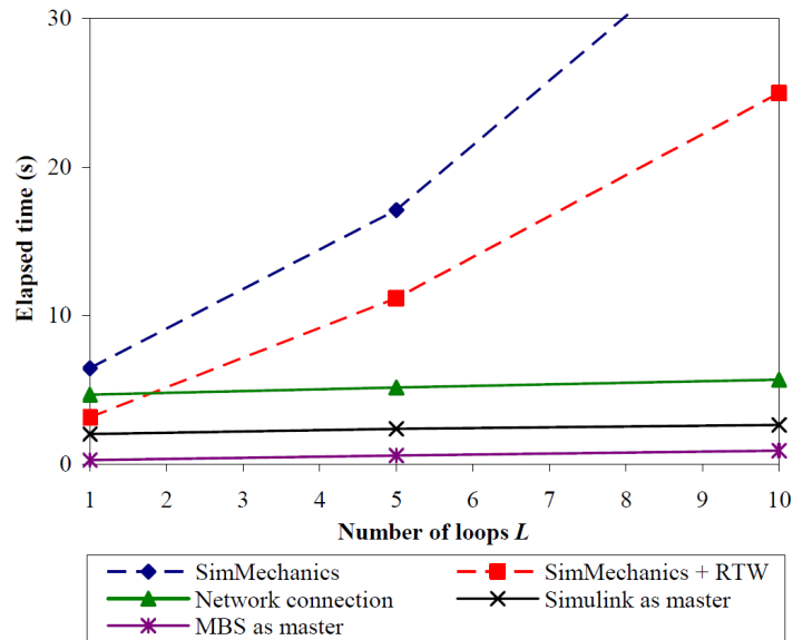
Figure 10: Elapsed times for a 30 s simulation of the L -loop linkage powered by the engine, with different simulation techniques
