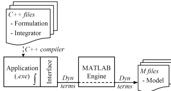
Figure 4: Function evaluation configuration with MATLAB Engine
