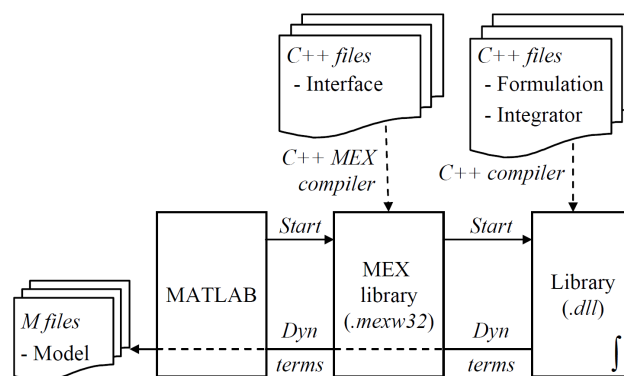
Figure 6: Function evaluation configuration with MEX API of functions
