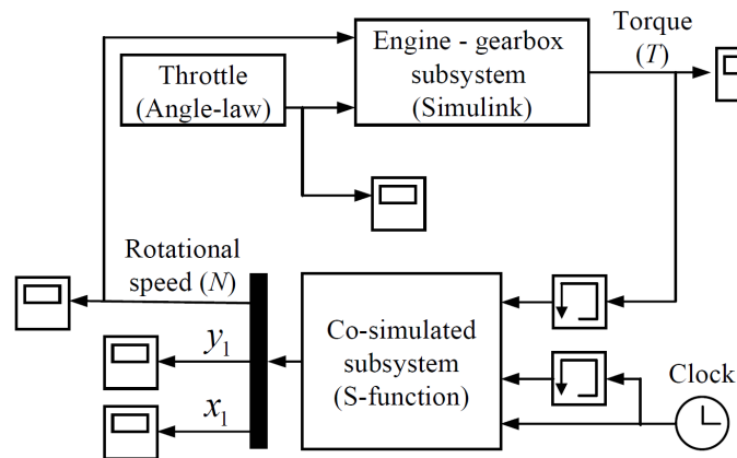
Figure 8: Simplified Simulink model for co-simulation, implemented with an S-function
