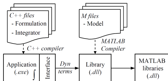
Figure 5: Function evaluation configuration with MATLAB Compiler
