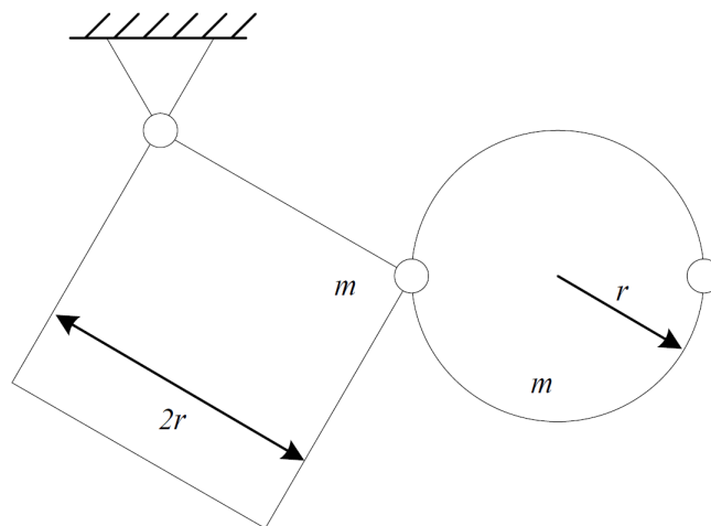
Figure 3: Double pendulum
