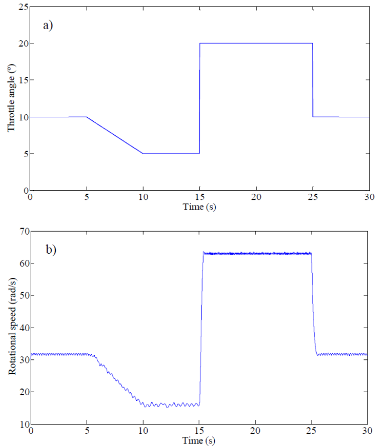
Figure 9: Throttle angle (a) and rotational speed of the mechanism (b) for a 30 s simulation of a 1-loop linkage
