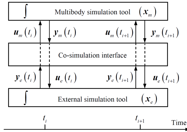
Figure 2: Generic co-simulation configuration
