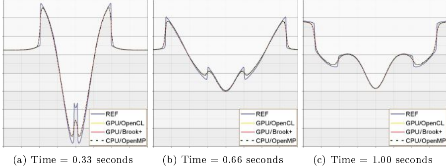
Figure 8: Evolution of the academic 2D problem used for verification.
