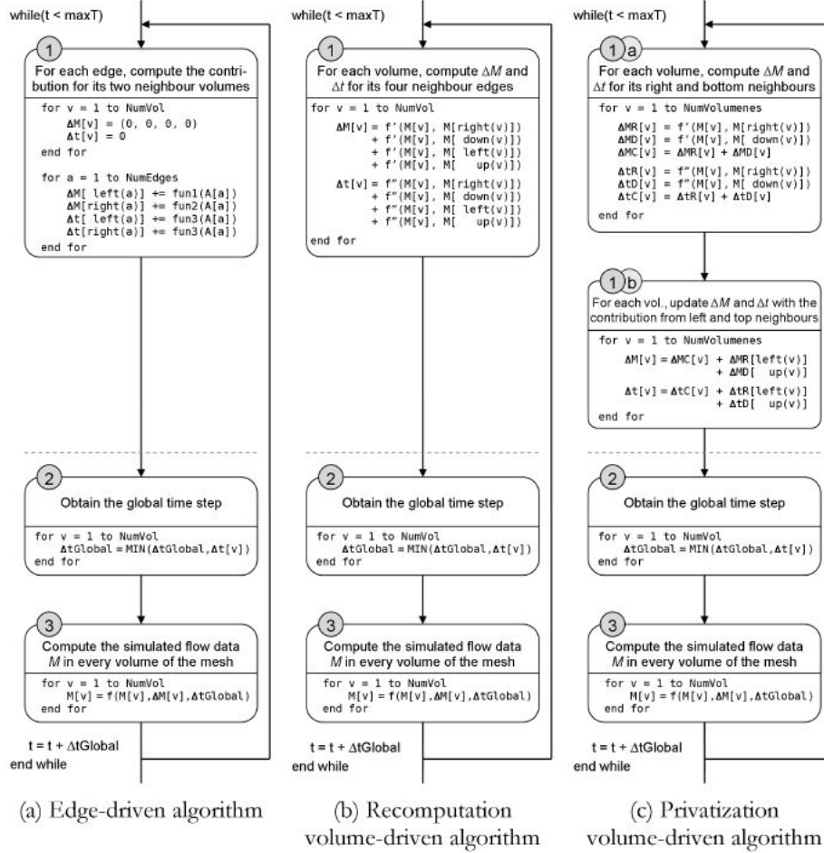
Figure 3: Diagram comparing the studied implementations.
