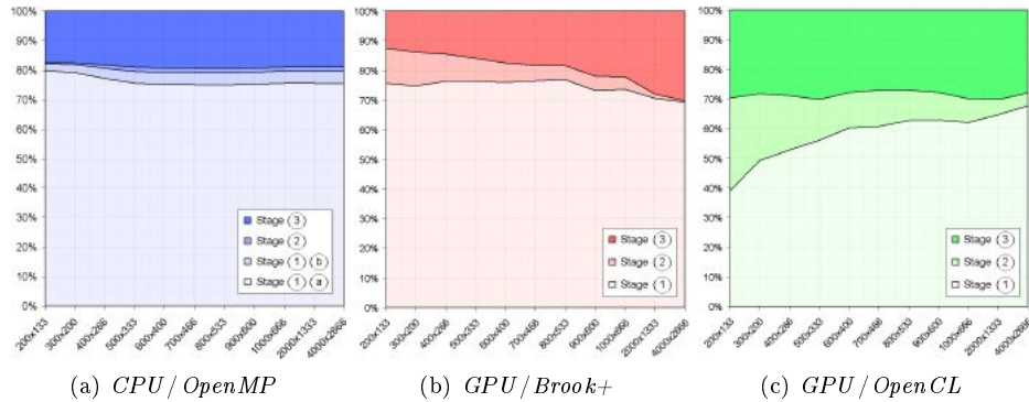
Figure 12: Relative computational cost of each stage of the algorithm.
