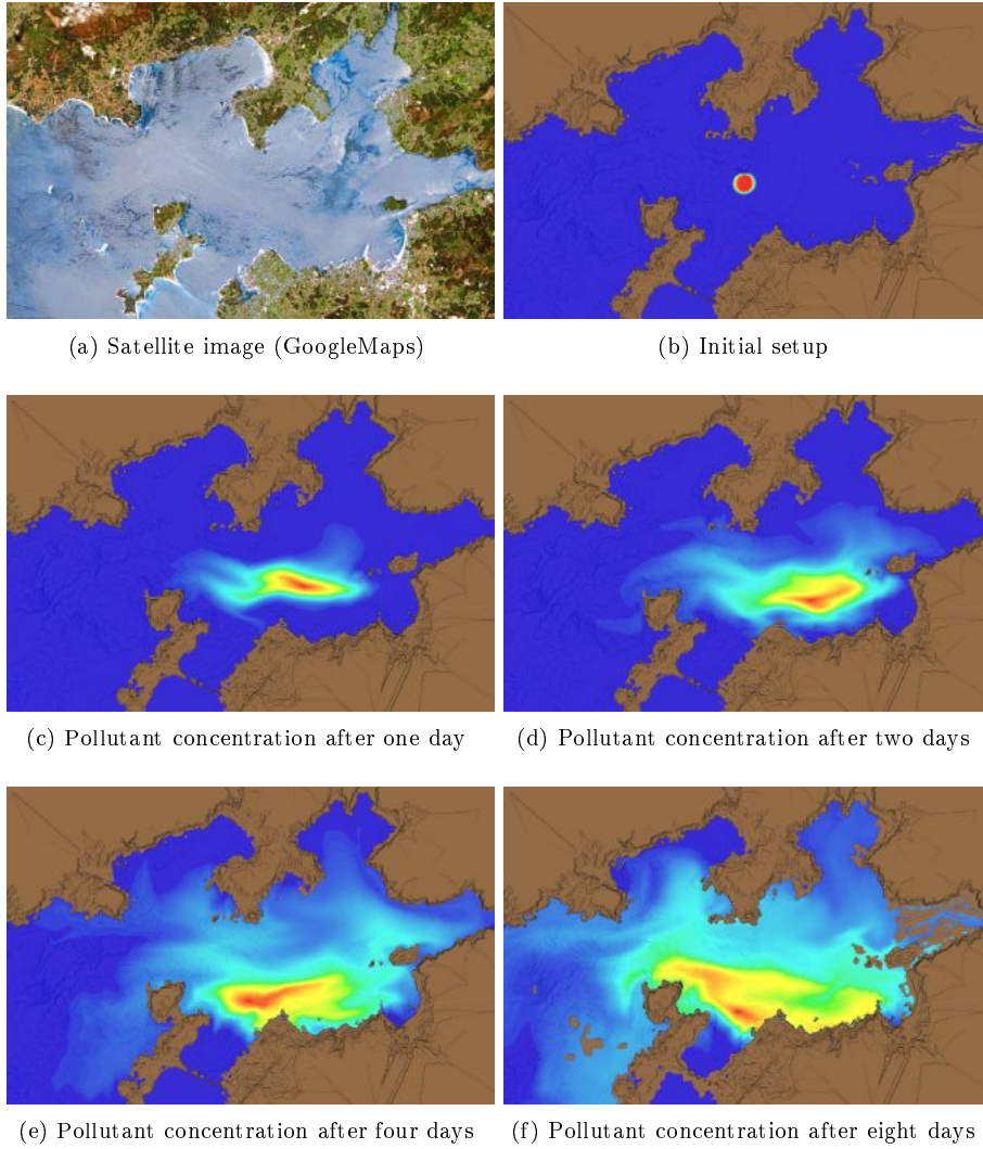
Figure 9: Evolution of the Ría de Arousa simulation.
