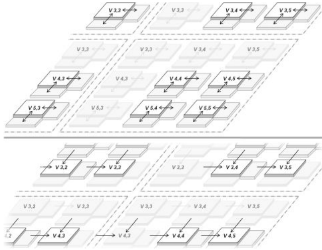
Figure 5: Optimized privatization volume-driven algorithm with block border replication.
