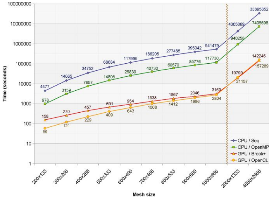
Figure 10: Execution time (in seconds) for several mesh sizes.
