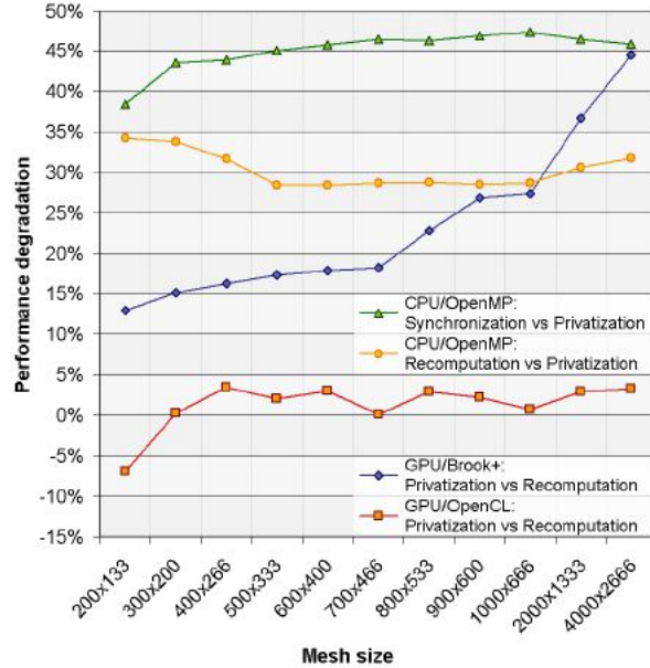
Figure 6: Pairwise comparison of the different parallelization strategies for each platform.
