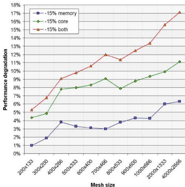
Figure 11: Performance impact of the GPU core and memory clock frequency on performance.
