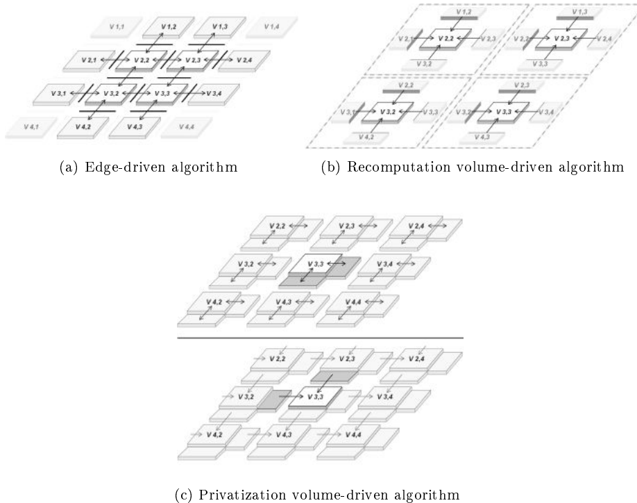
Figure 4: Parallelization strategies evaluated in this work.
