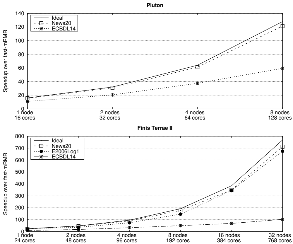
Figure 3: Speedups of fast-mRMR-MPI over fast-mRMR selecting 200 features of the largest datasets.
