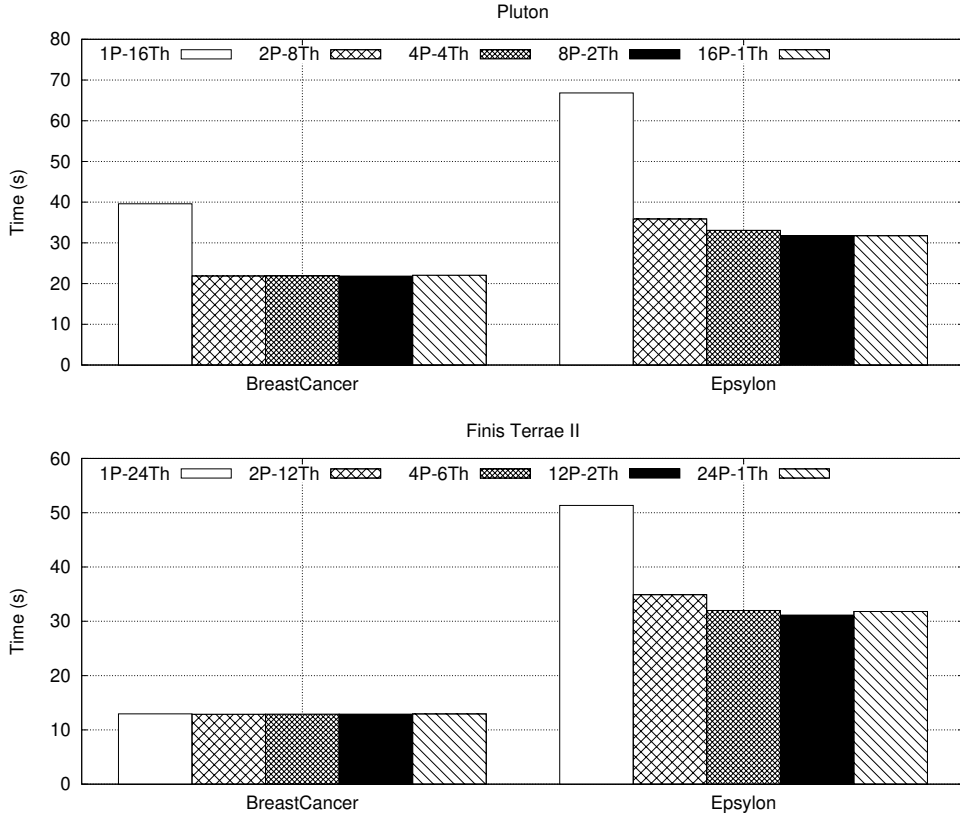
Figure 2: Runtime of fast-mRMR-MPI on one node of each platform when selecting 200 features of BreastCancer and Epsilon ( P=\#\text{processes} ; \text{Th}=\#\text{threads per process} ).
