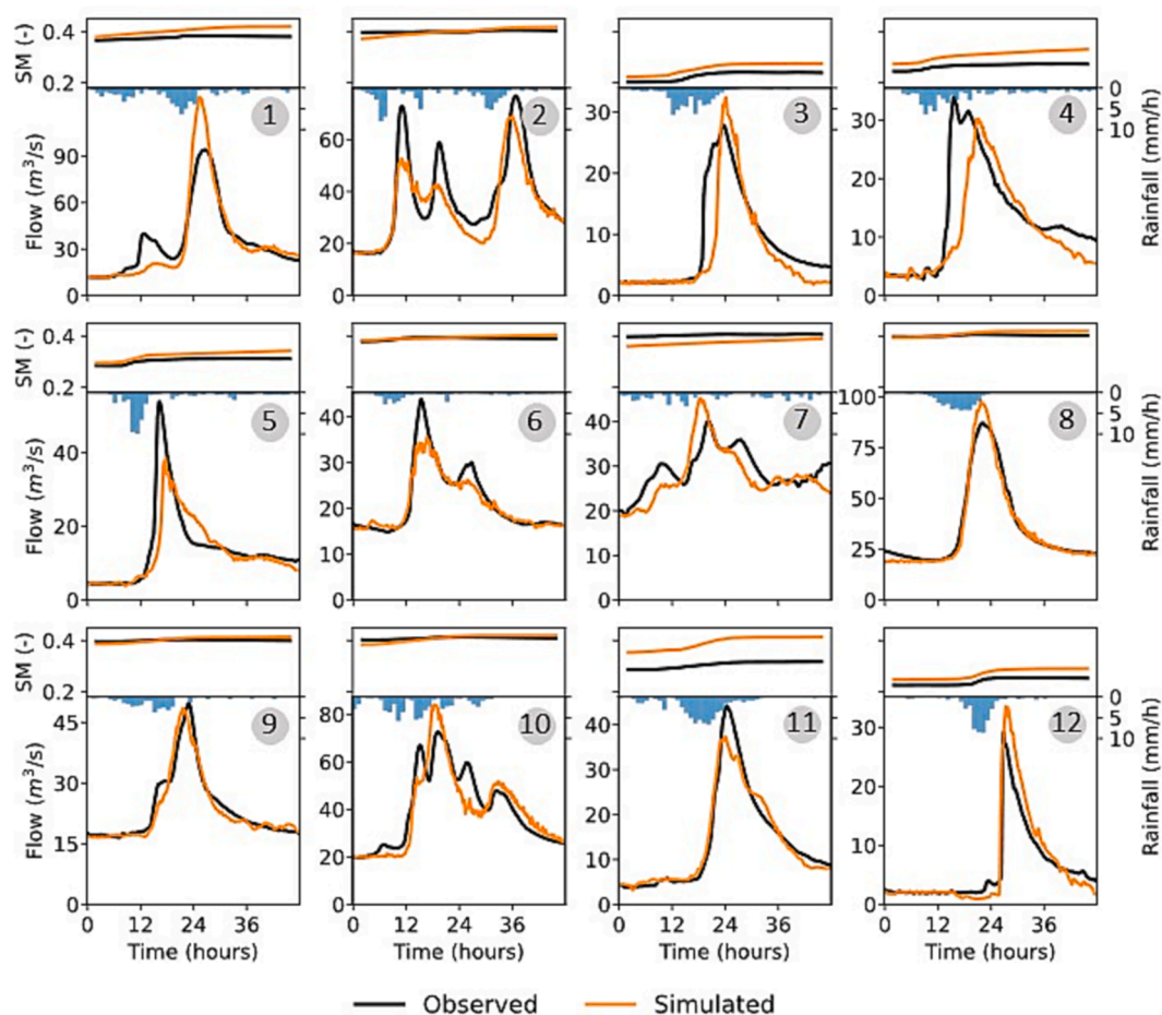
Fig. 12. Result of observed (black) and simulated (orange) hydrographs after the joint assimilation of discharge and soil moisture in the second application of the TPF approach. (For interpretation of the references to colour in this figure legend, the reader is referred to the web version of this article.)
