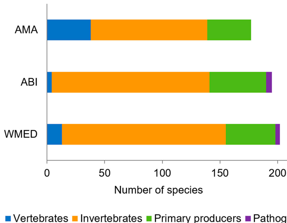
Figure 2. Number of introduced species detected by 2021 in Spanish marine waters included in the subregions WMED = Western Mediterranean, ABI = Bay of Biscay–Iberian Shelf, and AMA = Macaronesia.
