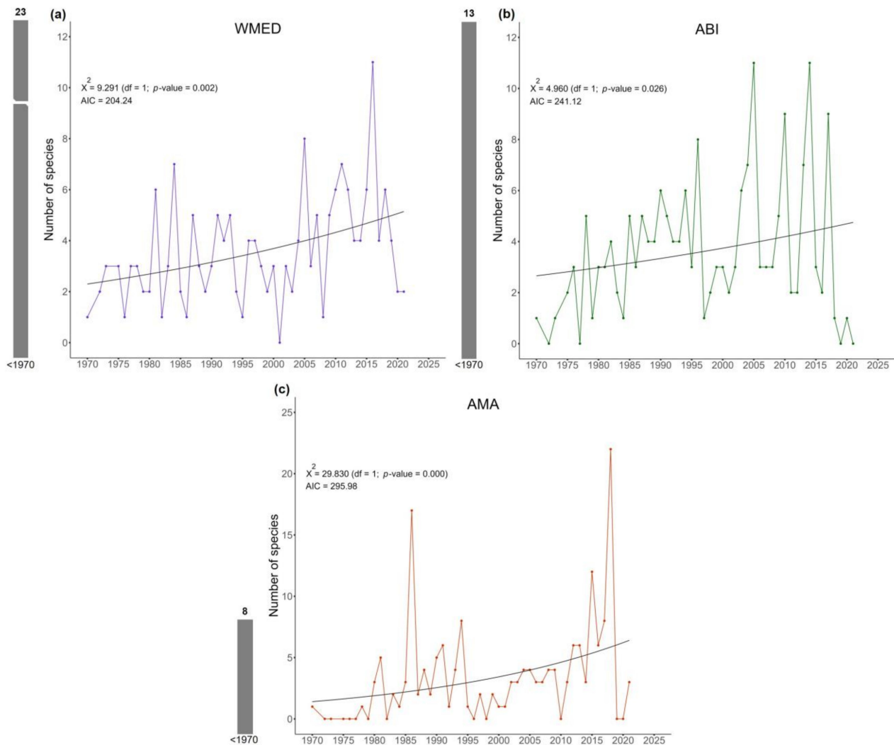
Figure 4. Temporal trend in newly introduced species for Spanish marine waters in (a) WMED = Western Mediterranean, (b) ABI = Bay of Biscay–Iberian Coast, and (c) AMA = Macaronesia. The black line represents the GLM model output. The grey bar shows the amount of introduced species before 1970.
