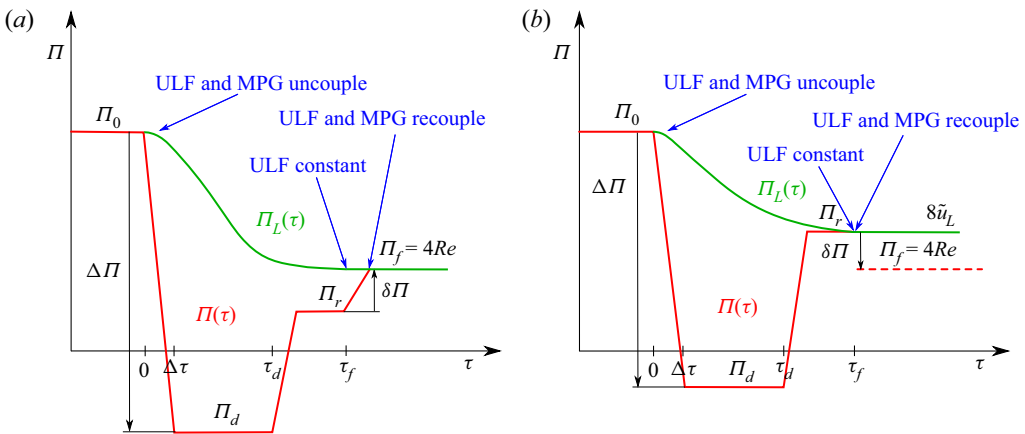
Figure 7. Laminalisation pattern: sketch of MPG \Pi(\tau) evolution in the core flow for the annular jet and radial jets experiments. Here \Pi_L(\tau) is a virtual MPG, corresponding to the laminar Hagen–Poiseuille flow that at each instant has the same Re_L as the U-ULF. (a) Successful complete laminalisation ( \Pi_r < \Pi_f = 4Re ); (b) unsuccessful complete laminalisation ( \Pi_r > \Pi_f = 4Re ).
