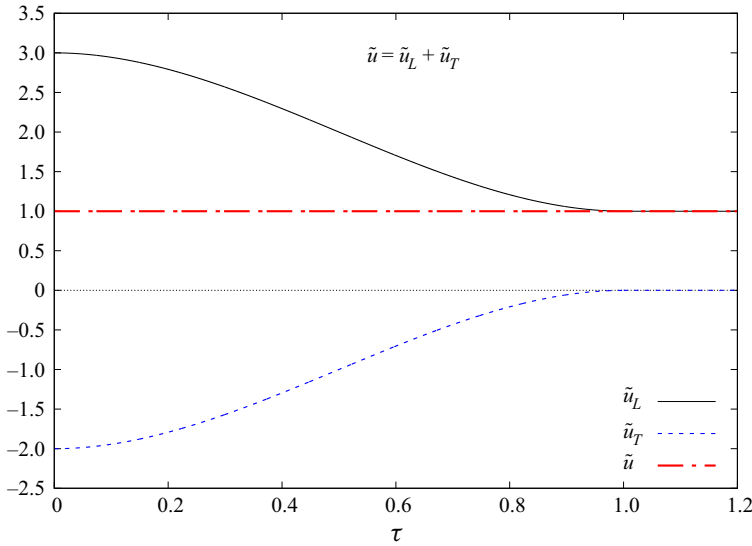
Figure 4. Evolution of \tilde{u}_L and \tilde{u}_T after a sufficiently low MPG (in arbitrary units, \tilde{u} = \tau_f = 1 ). Each variation in \tilde{u}_L must be matched by an equal and opposite variation in \tilde{u}_T .
