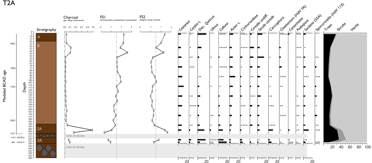
Fig. 7. Synthetic figure summarising the main geochemical and palynological properties of T2A and T1C sequences.
