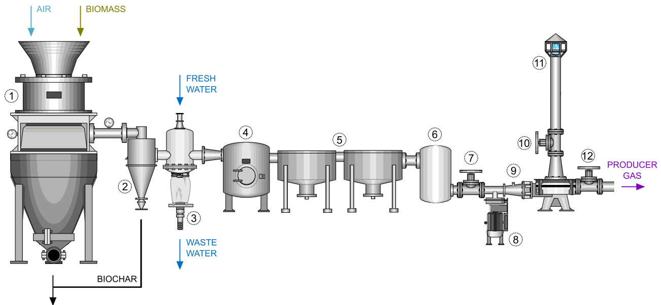
Fig. 1 – Layout of the experimental gasification plant. (1) Downdraft gasifier; (2) cyclone; (3) Venturi scrubber; (4) coarse particle filter; (5) fine particle filters; (6) bag filter; (7) control valve; (8) blower; (9) producer gas sampling point; (10) flare valve; (11) flare stack; (12) discharge valve.
