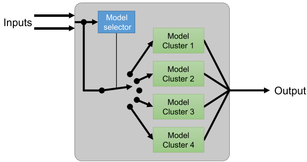
Fig. 4 – Internal configuration of the hybrid intelligent model.
