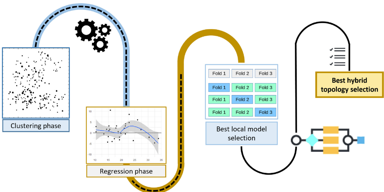
Fig. 5 – Flowchart to create the hybrid intelligent model.
