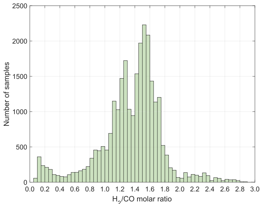
Fig. 6 – Histogram of the H 2 /CO molar ratio in the producer gas.
