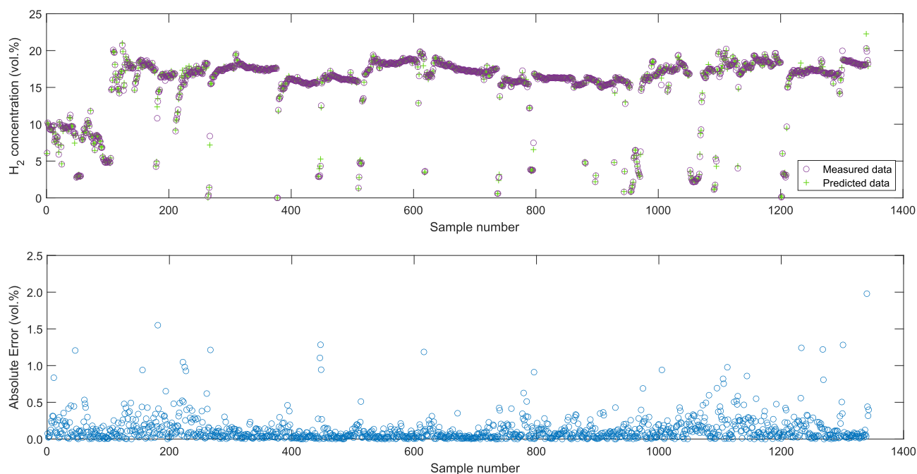
Fig. 8 – Scatter plots of the hydrogen concentration prediction test. Upper subplot: measured data (purple circles) and predicted data (green crosses). Lower subplot: absolute error (blue circles). (For interpretation of the references to color in this figure legend, the reader is referred to the Web version of this article.)
