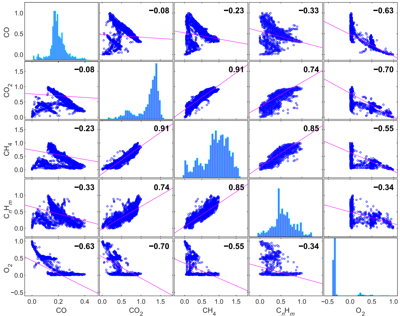
Fig. 7 – Pearson correlation matrix between all pairs of input variables to the hybrid intelligent model.
