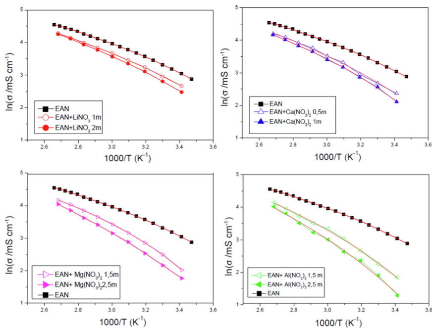
Fig. 10. Arrhenius plots for the conductivities of pure EAN (data taken from Ref. [53]) and its mixtures with LiNO 3 (a), Ca(NO 3 ) 2 (b), Mg(NO 3 ) 2 (c) and Al(NO 3 ) 3 (d) near the solubility limit and at an intermediate concentration. The red lines shown in the plot correspond to the fitting to the VFT Eq. 3 (parameters shown in Table 2).
