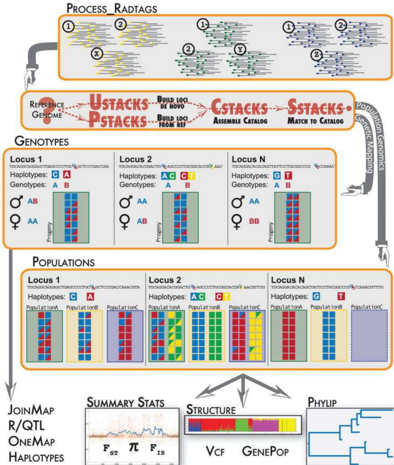
Figura 2. Pipeline de STACKS [2]
