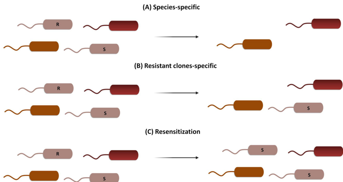
Figure 2. Three different CRISPR-Cas strategies to combat AMR. (A) Species-specific targeting kills both susceptible and resistant clones of the same species, leaving the rest of the microbial population unaltered. (B) Resistant clones-specific targeting kills only bacteria harboring genes for AMR, leaving susceptible clones and the rest of the population unaffected. (C) Resensitization turns resistant clones into susceptible ones by specifically targeting resistance genes, without an effect on the rest of the microbial population.
