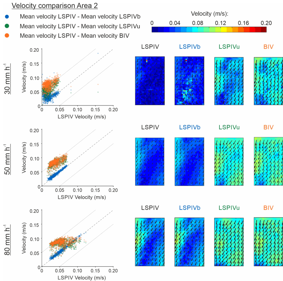
Figure 7. Velocity comparison between imaging velocimetry techniques results (LSPIV, LSPIVb, LSPIVu, and BIV) in Area 2 for the three different rain intensities (30, 50, and 80 \text{ mm h}^{-1} ). The velocity fields obtained for each case are also plotted for a qualitative comparison.
