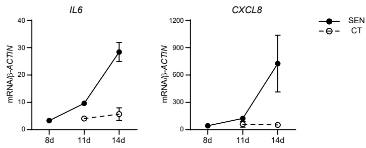
Fig. S2. Kinetics of IL6 and CXCL8 mRNA expression in senescent SF.
