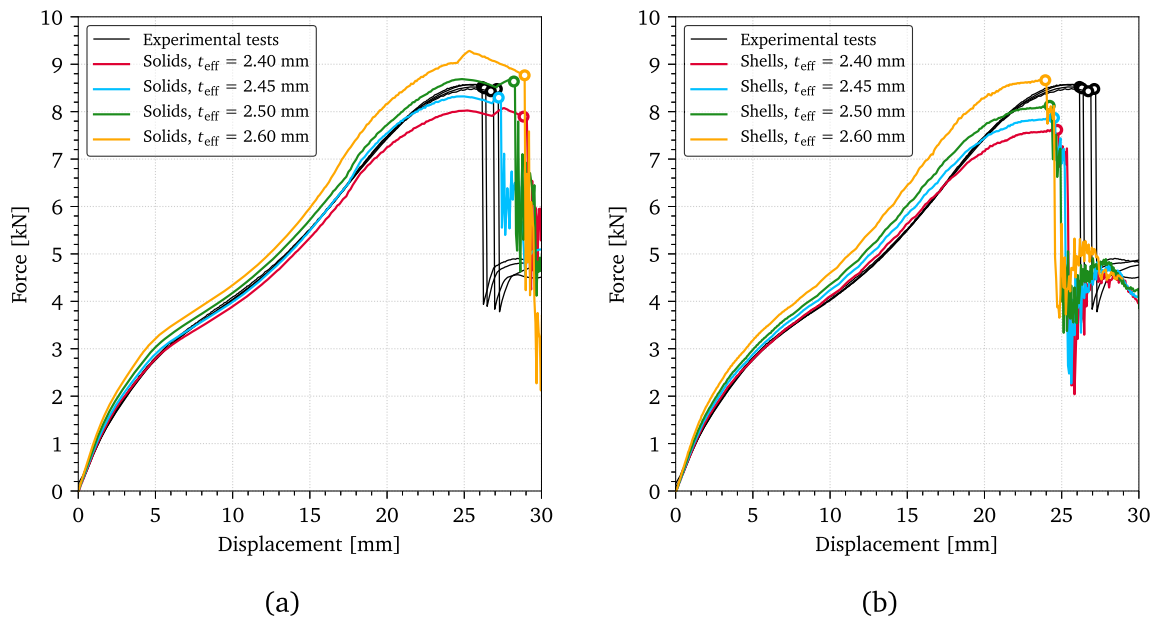
Fig. 17. Influence of the effective thickness t_{\text{eff}} on the force–displacement curves of the component tests simulated with solid elements (a) and shell elements (b).
