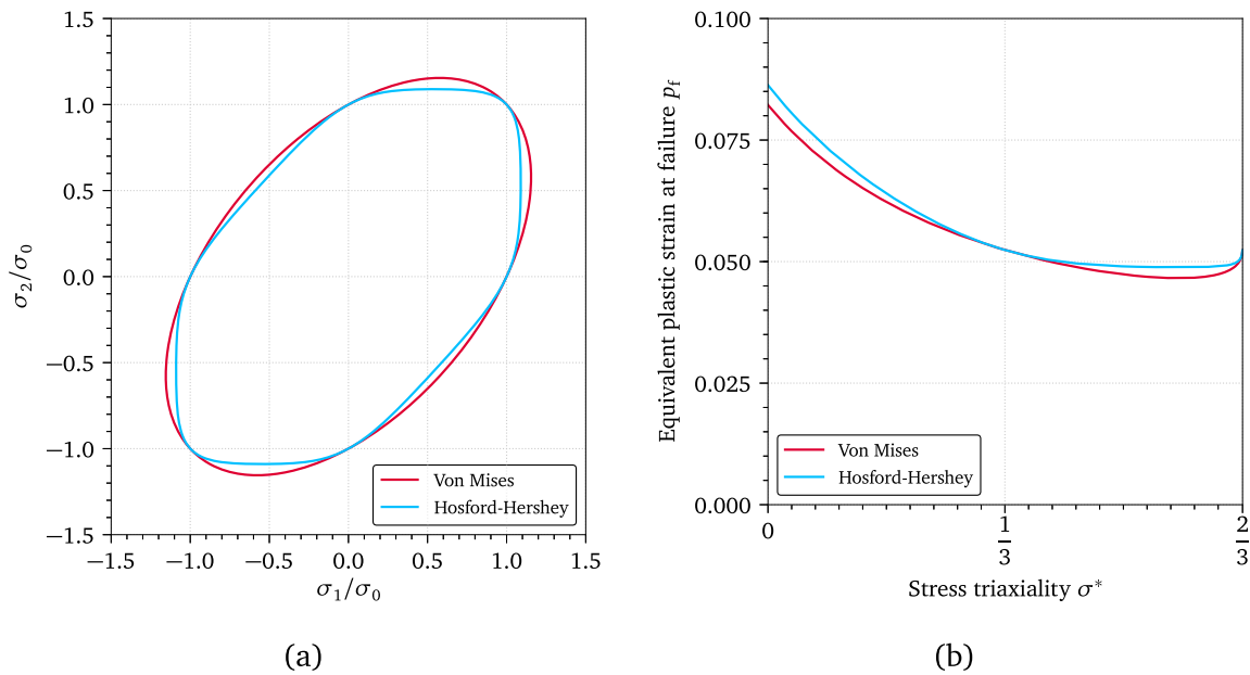
Fig. 14. Comparison of the von Mises and Hershey yield surfaces (a) and the fracture loci of the Cockroft–Latham criterion adopting one or another surface for the material calibrated at 90 degrees with the printing direction (b). Plane stress conditions are assumed in both figures.
