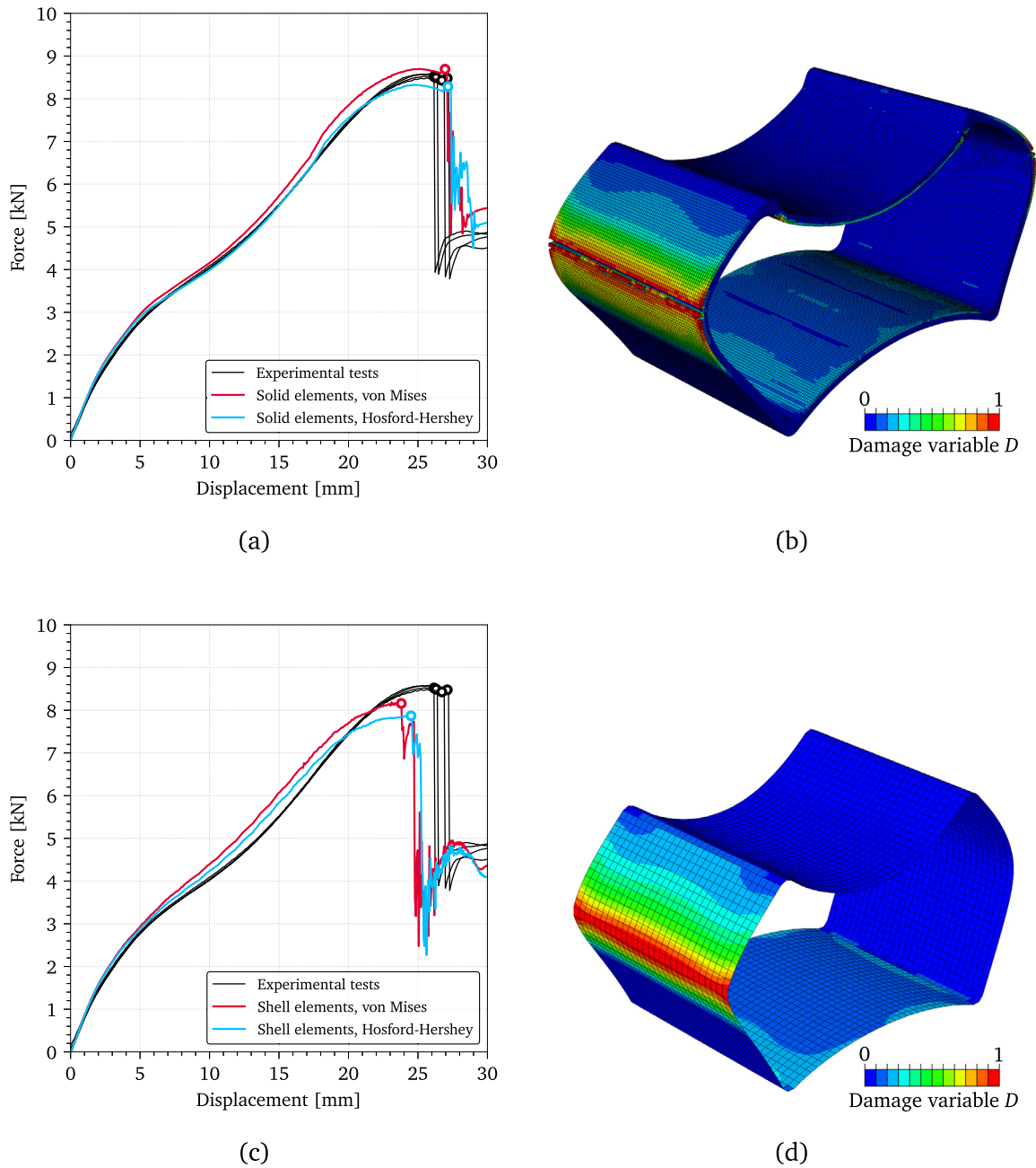
Fig. 12. Results of the simulations of the component tests: force–displacement curves with solid elements (a) and deformed shape at failure (b), and force–displacement curves with shells (c) and deformed shape at failure (d). Dots indicate failure.
