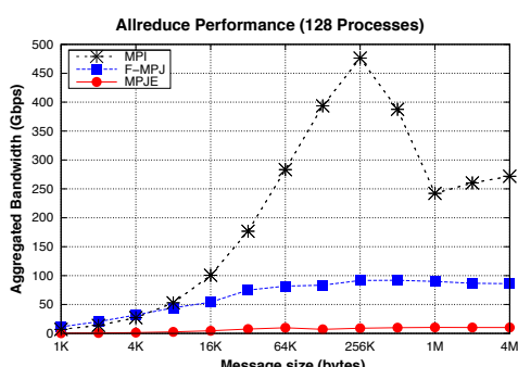
Figure 5: Collective primitives performance on the InfiniBand multi-core cluster
