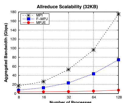
Figure 5: Collective primitives performance on the InfiniBand multi-core cluster
