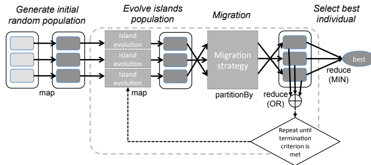
Fig. 1: Island-based parallel DE implementation using Spark.
