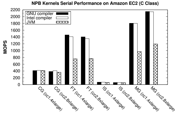
Figure 5: NPB kernels serial performance
