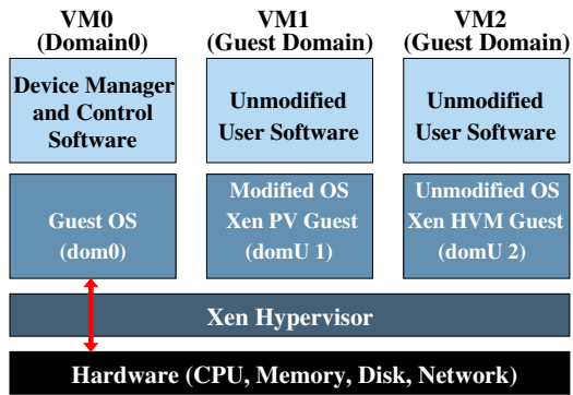
Figure 1: Xen architecture overview
