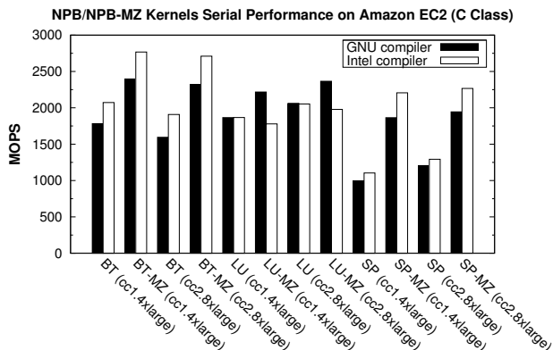
Figure 10: NPB/NPB-MZ kernels serial performance
