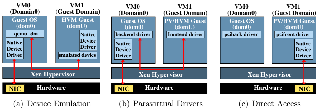
Figure 2: Network virtualization support in Xen
