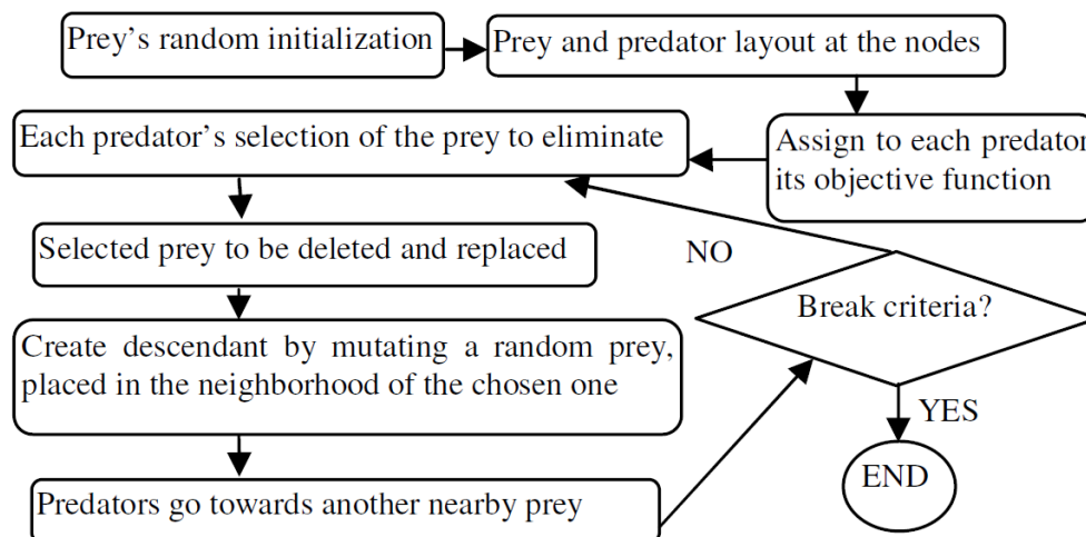
Fig. 2 Operation diagram of the predator-prey approach
