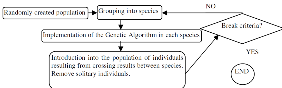
Fig. 1. Operation diagram of grouping into species
