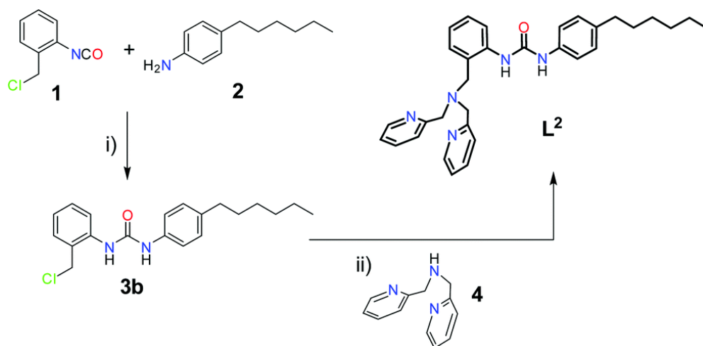
Scheme 2. Synthesis of L^2 . Reagents and conditions: (i) Et 2 O, r.t., 48 h; (ii) CH 3 CN, dipea, KI (cat.), Δ, 72 h.
