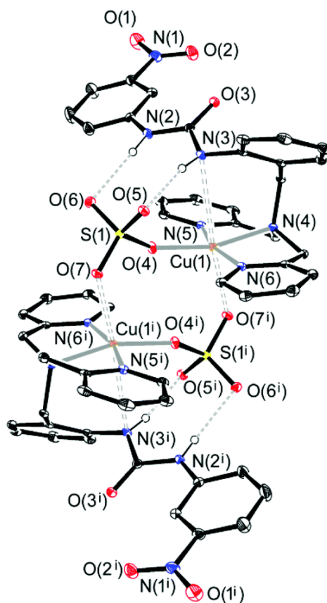
Fig. 4. View of the X-ray structure of [CuL 1 (μ-SO 4 ) 2 ]. Hydrogen atoms bonded to carbon atoms are omitted for clarity.
