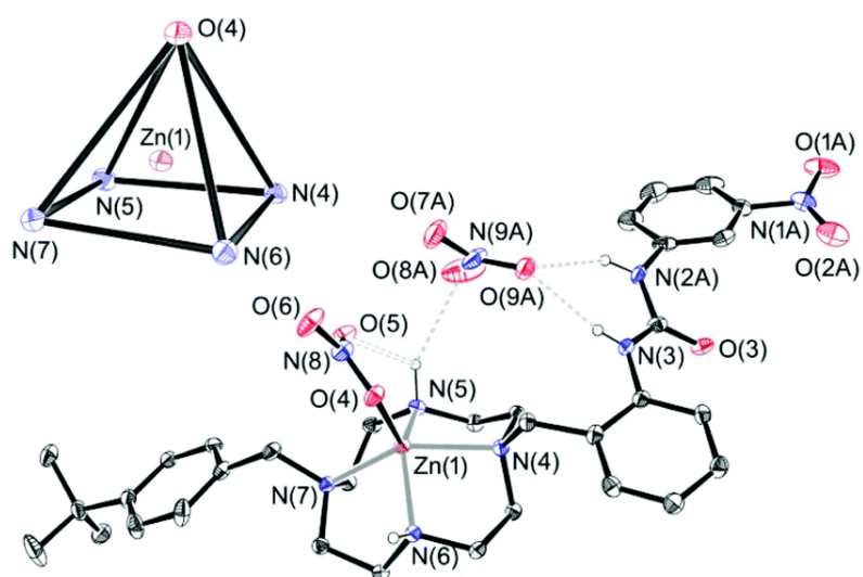
Fig. 3. The X-ray structure of [ZnL 3 (NO 3 )](NO 3 ). Hydrogen atoms bonded to carbon atoms are omitted for clarity. The inset shows a representation of the square pyramidal coordination polyhedron. The uncoordinated nitrate ion and the distal part of the urea moiety show positional disorder with occupation factor of 0.613(8) for atoms labelled with A.
