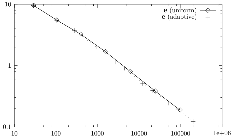
Figure 5.1.2: e vs. N for both refinements (Example 1, \alpha = 10 , \nu = 1 ).
