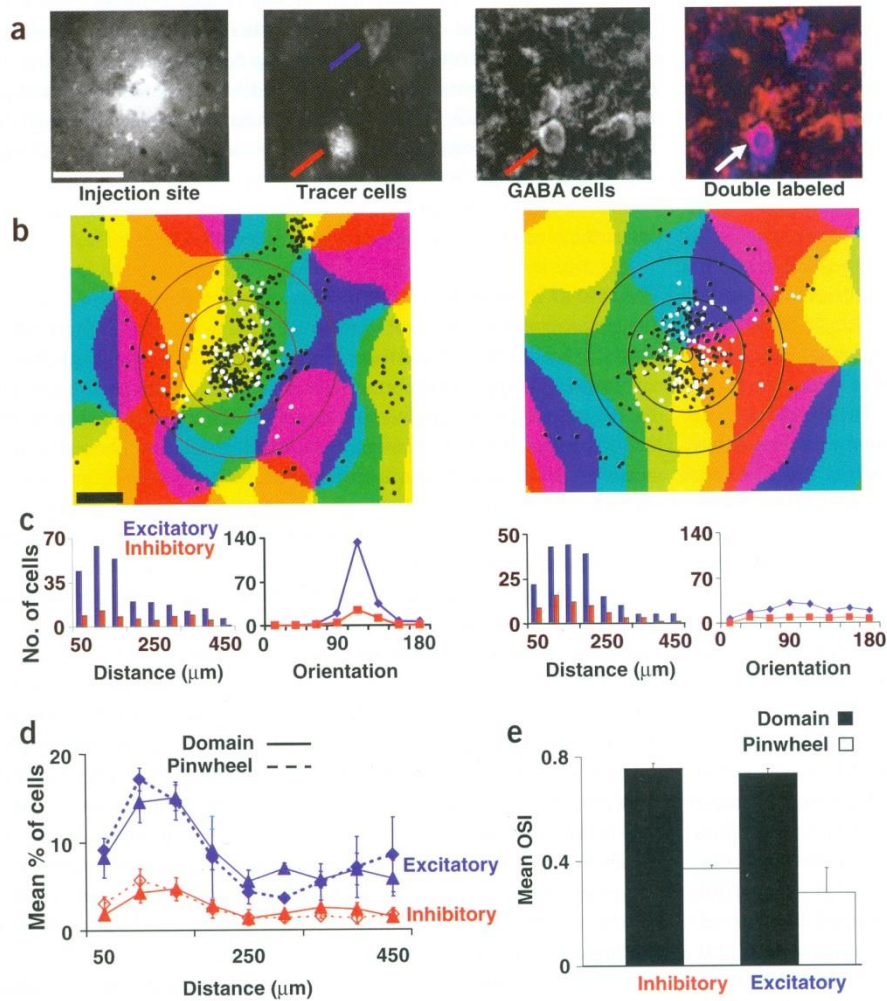
Figure 4 Anatomical analysis of local excitatory and inhibitory projections to pinwheel centers and orientation domains. (a) Example of an injection site (see le bar: 100 \mu\text{m} ), and three images of the same region showing retrogradely labeled, GABA-positive and double-labeled cells, respectively. For illustration purposes, the two middle images were high-pass filtered and merged to show the double-labeled neurons at right. (b) Examples of the distribution of cells within the orientation map following an injection of tracer in an orientation domain (left) and a pinwheel center (right). Black: excitatory cells; white: inhibitory cells. The two outer concentric circles are at 250- \mu\text{m} intervals from the injection site (inner circle). Scale bar: 250 \mu\text{m} . (c) Histograms and tuning curves computed from the orientation domain (left) and pinwheel (right) cells depicted in b. Histograms show the number of inhibitory and excitatory cells located at different distances from the injection. The orientation tuning curves indicate the number of inhibitory and excitatory cells found in the different orientation regions, within a distance of 250 \mu\text{m} . (d) Population curves of three pinwheel and four domain injections showing the proportion of inhibitory and excitatory cells found at different distances from the injection. (e) Bar plot of the mean OSIs for the population data. Error bars in d and e show s.e.m.
