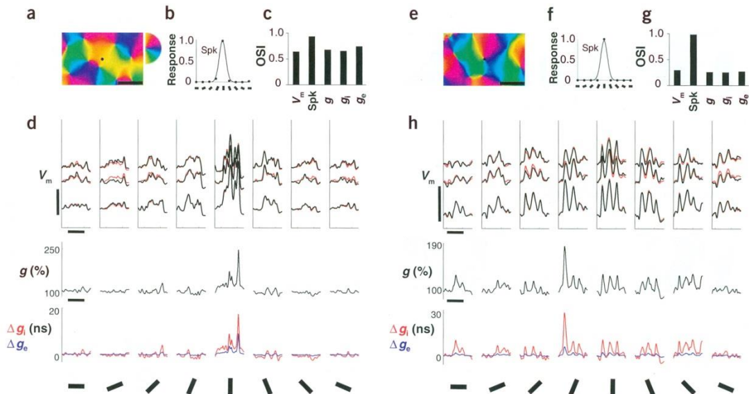
Figure 1 Orientation tuning of synaptic conductances for a cell in an orientation domain ( a-d ) and at a pinwheel center ( e-h ). ( a,e ) Orientation preference maps from VI (a small region is shown, from a large region that was imaged). Filled circles indicate the location of recording electrodes. Color-coded semicircle in a indicates the angle of orientation preference of each pixel. Scale bars. 500 \mu\text{m} . ( b,f ) Orientation tuning curves of the spike responses. ( c,g ) OSIs calculated for the membrane potential ( V_m ), spike response (Spk), total conductance ( g ) and inhibitory and excitatory conductances ( g_i and g_e ). V_m and the underlying conductances ( g , g_i and g_e ) are relatively narrowly tuned for the orientation domain cell but are broadly tuned for the pinwheel center cell. Spike tuning is invariantly sharp for both cells. ( d,h ) Traces of the average visually evoked changes in V_m , g , g_i and g_e in response to each of eight stimulus orientations spanning 180°. (Top rows) V_m traces. Black lines show the mean activity for three to five trials under resting conditions and for two levels of current injection (-0.2 and 0.1 nA). Red lines show the predicted V_m traces from linear regression fits used to obtain g (see Methods). The predicted and actual traces are in good agreement. Horizontal scale under g , 1 s (visual stimulation time); vertical scale, 10 mV in d and 5 mV in h . (Middle rows) g traces showing changes relative to rest. (Bottom rows) \Delta g_i and \Delta g_e traces showing absolute changes in g_i and g_e .
