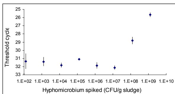
Figure 4. Threshold cycle ( C_T ) versus the amount of Hyphomicrobium VS spiked in the sludge samples (n=3).
