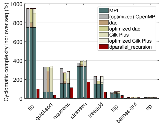
Fig. 13 Cyclomatic complexity comparison
