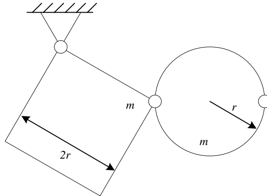
Figure 5.4: Double pendulum
