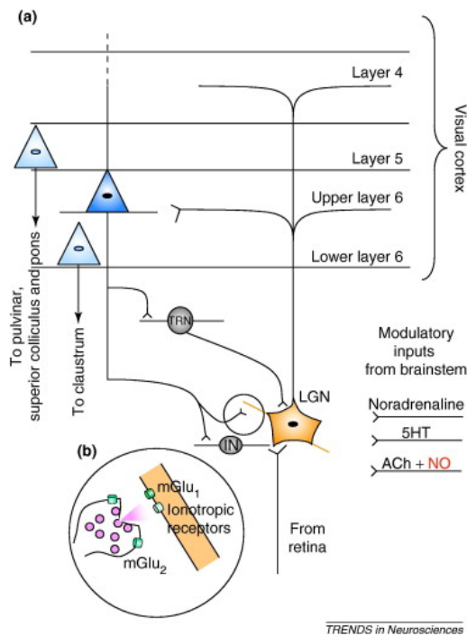
Figure 1. Corticogeniculate circuitry of cats. (a) Thalamocortical axons have dense terminals in cortical layer 4 (with sparser extensions in layers 1 and 3; not shown) and give branches to layer 6. Lateral geniculate nucleus (LGN) relay cells receive, together with the specific visual input from the retina, multiple neuromodulatory inputs from the brainstem, and massive corticogeniculate feedback from cells located in upper layer 6 (dark blue). This input is glutamatergic and employs both ionotropic and metabotropic receptors. A collateral axon branch to the thalamic reticular nucleus (TRN) and an intrinsic inhibitory interneuron (IN) are also illustrated. There are other afferents to the LGN not shown in this figure: cells of the optic tract nucleus in the midbrain and of the tuberomammillary nucleus in the hypothalamus provide GABAergic and histaminergic inputs, respectively. In cats, the visual part of the TRN is known as the perigeniculate nucleus [6]. (b) A magnified representation of corticogeniculate terminals, illustrating postsynaptic ionotropic and mGlu 1 metabotropic receptors and presynaptic mGlu 2 metabotropic receptors, which are known to operate in the cat LGN.
