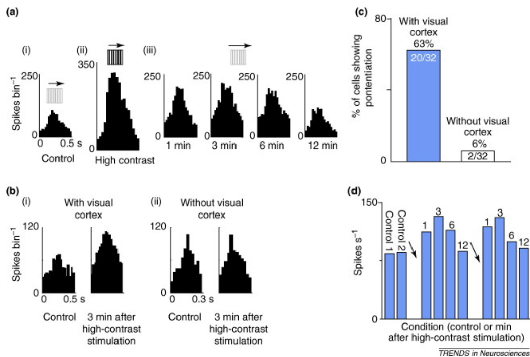
Figure 3. Cortical feedback influences LGN activity in the temporal domain. (a) The effect of high-contrast stimulation on subsequent visual responses. PSTHs were obtained under control conditions (i.e. stimulation using a low-contrast stimulus) and following visual stimulation using high-contrast stimulus (ii). Responses were then measured again using low-contrast stimulation 1, 3, 6 and 12 min after the end of high-contrast stimulation (iii). (b) PSTHs from two cells recorded during the same experiment before (i) and after (ii) decortication. (c) Summary of potentiation responses for the population of cat cells studied with and without corticofugal input. (d) Single-cell data from a magnocell in the macaque LGN. The augmentation effect obtained by 1 min exposure to a high-contrast drifting grating (arrow) was reproducible in a second period of stimulation following recovery. Modified, with permission, from Ref. [69] © (2000) Blackwell Publishing Group.
