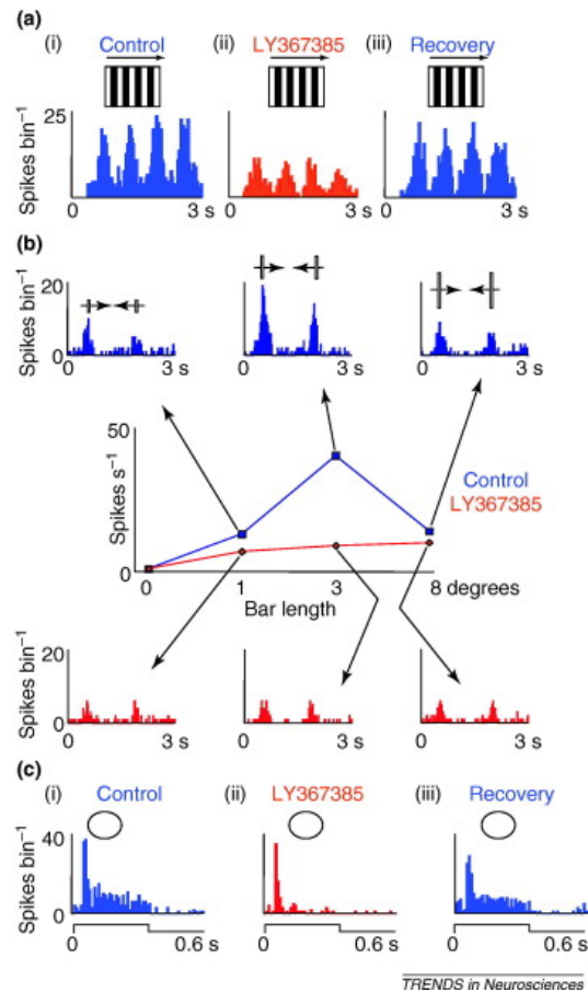
Figure 2. Cortical influence mediated by mGlu 1 receptors in anaesthetised cats. (a) Peristimulus time histograms (PSTHs) illustrate the response of the cell to a full-field sinusoidal drifting grating (illustrated above the PSTHs) of optimal characteristics under control conditions (i), in the presence of the specific mGlu 1 antagonist LY367385 (ejected iontophoretically using 60 nA for 6 min; ii), and after a recovery period of 15 min (iii). (b) Length-tuning curves constructed for a bar of varying length moving in both directions (illustrated above the PSTHs) over the receptive field. The blue curve is the control response; the red curve is the response during LY367385 application (6 min, 60 nA). PSTHs are shown for each bar length. It is clear that the response decreases when the mGlu 1 antagonist is applied. The strongest effect is seen for the optimal length (3° in this example). (c) Transient responses are not affected by mGlu 1 blockade. PSTHs show the response of an LGN cell to flashed spots (represented by the circle above the PSTHs) restricted to receptive-field centre, before (i), during (ii) and after (iii) application of the specific mGlu 1 antagonist (ejection: 80 nA, 3 min). Only the sustained part of the response was reduced by the antagonist. Modified, with permission, from Ref. [31] © (2002) the Society for Neuroscience.
