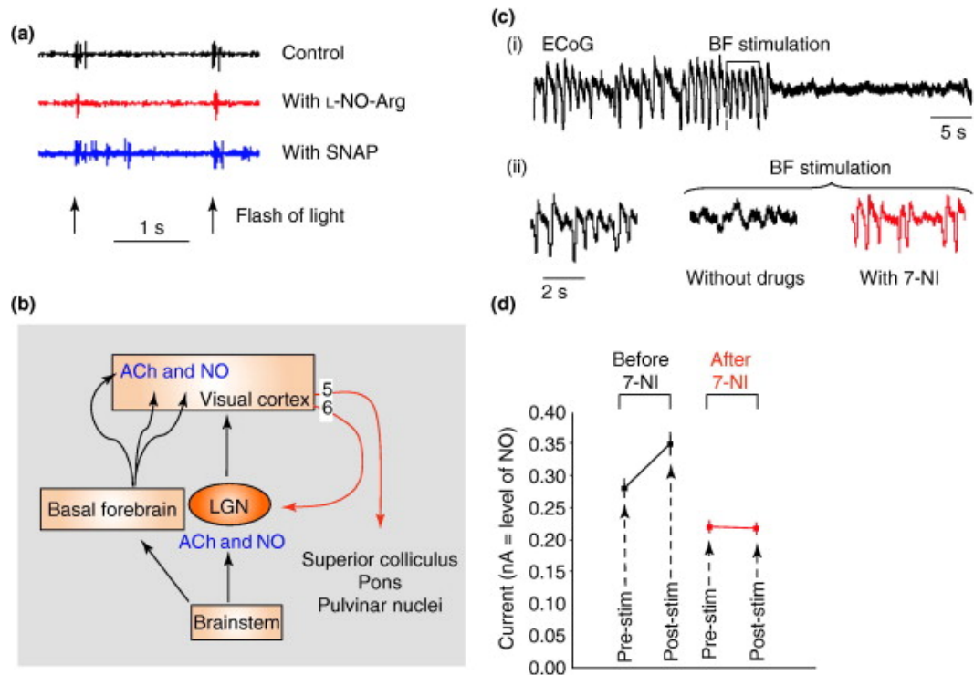
Figure 4. Modulation of nitric oxide (NO) synthesis produces changes in thalamic and cortical neuronal activity. (a) The thalamic effect of NO: control responses to an optimum flashed stimulus (black); the effect of blockade of NO using L-NO-Arg (red); and the effect of NO augmentation using SNAP (an NO donor, blue). (b) The basal forebrain (BF)–cortical loop. The BF receives various inputs from the brainstem (noradrenergic, serotonergic, cholinergic and dopaminergic inputs) that are considered important modulators of the sleep–wake cycle and behavioural arousal. Cholinergic neurons of the BF are widely hypothesized to modulate the level of arousal or activation in various limbic structures and cortical sites. There are well documented monosynaptic projections of BF cholinergic neurons to the neocortex, including connections that form part of the visual system (the BF also receives cortical feedback, which originates from a restricted portion of the cortex, including prefrontal, insular, and piriform cortices; not shown) 73, 81 and 83. Interestingly, these ACh-containing fibres also contain NO synthase. Cortical activation due to ACh and NO release would increment the gain of the corticofugal feedback (red arrows) from layer 6 to the LGN, and also from layer 5 to the superior colliculus, the pons and higher-order thalamic regions such as the pulvinar complex; these regions occupy an analogous position in the extrastriate visual system to the LGN in the primary visual pathway, but deal with higher-order visual and visuomotor transduction. (c) (i) Electroencephalogram (ECoG) activity recorded in the visual (V1) cortex before, during and after electrical stimulation of the BF for 4 s (horizontal line). This stimulation produced a change in ECoG from a sleep-like to a wake-like pattern. (ii) The ECoG in the control situation, and the patterns seen after BF stimulation without drugs and when the subject animal was given the NO synthase inhibitor 7-NI (red). (d) NO cortical levels as measured by voltammetry. The panel shows the mean and standard deviation of all data points recorded over the 8 h of the experiment in one cat. Data were obtained under two different conditions, before and after intraperitoneal application of 7-NI. For each condition, the values immediately before electrical stimulation were compared with those obtained immediately after stimulation. The observed changes are statistically significant only for the pre-drug condition. Panel (a) is modified, with permission, from Ref. [76] © (2000) the Associated Professional Sleep Societies, LLC; (c,d) are modified, with permission, from Ref. [80] © (2003) the Society for Neuroscience.
