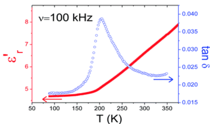
Fig. 3 Temperature dependence of the dielectric constant, \epsilon'_r , (solid squares) and the dielectric losses, \tan \delta , (open circles) of (\text{C}_3\text{N}_2\text{H}_5)[\text{Mn}(\text{HCOO})_3] measured at \nu = 100\text{ kHz} .
