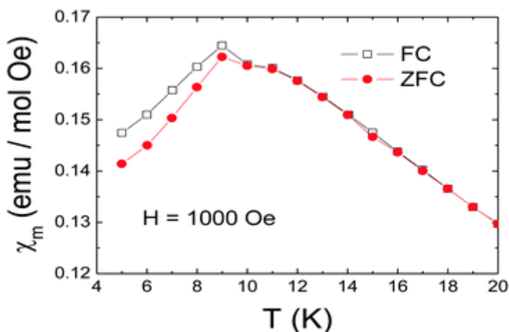
Fig. 6 ZFC-FC molar magnetic susceptibility of (\text{C}_3\text{N}_2\text{H}_5)[\text{Mn}(\text{HCOO})_3] measured under a high applied magnetic field H = 1000 \text{ Oe} .
