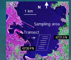
Figure 2. Location and sampling area in the Ria de A Coruña. The transect comprising 7 trap tows of the inner area is shown
