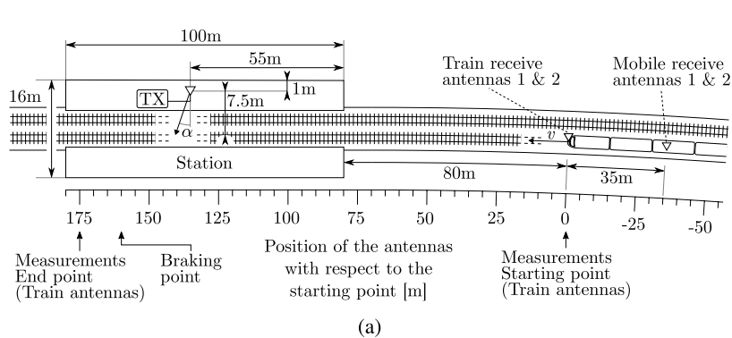
FIGURE 1. (a) Schematic of the measurement scenario (not at scale) at “La Almudena” subway station, Madrid Metro, Spain. The scenario consists of a modern subway station and its corresponding entrance tunnel. (b) Picture taken from the train cabin while conducting measurements. The train is at the measurement starting point with the station visible at the end.
