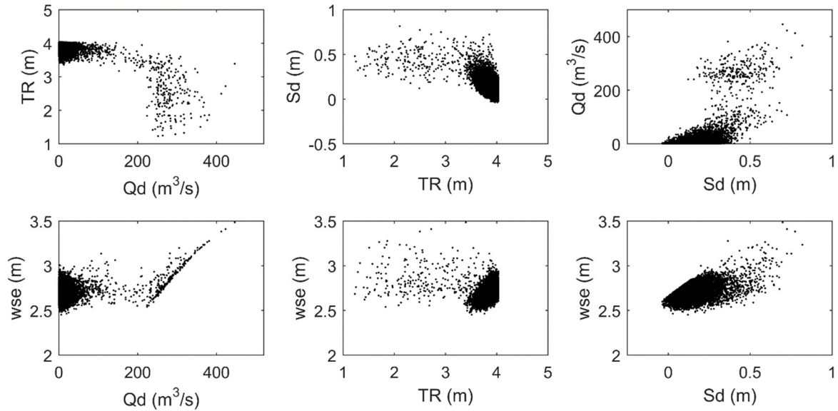
Figure 5. Annual maximum water surface elevation at control point 1 and associated daily peak discharge (Qd), astronomical tidal range (TR) and storm surge (Sd) conditions.
