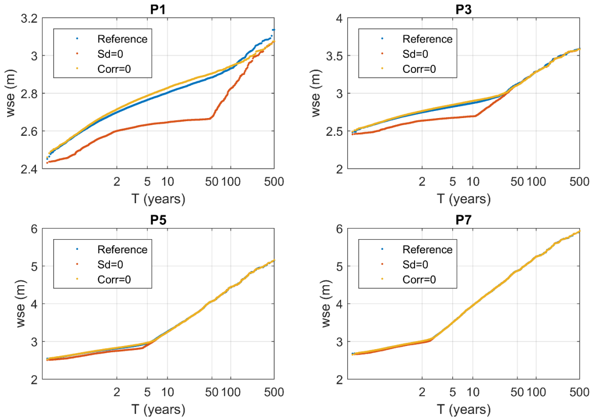
Figure 7. Water level frequency distribution obtained at points P1, P3, P5 and P7 with the original simulation (Reference), the simulation that neglects the storm surge (Sd=0) and the simulation that neglects the correlation between the storm surge and the river discharge (Corr=0).
