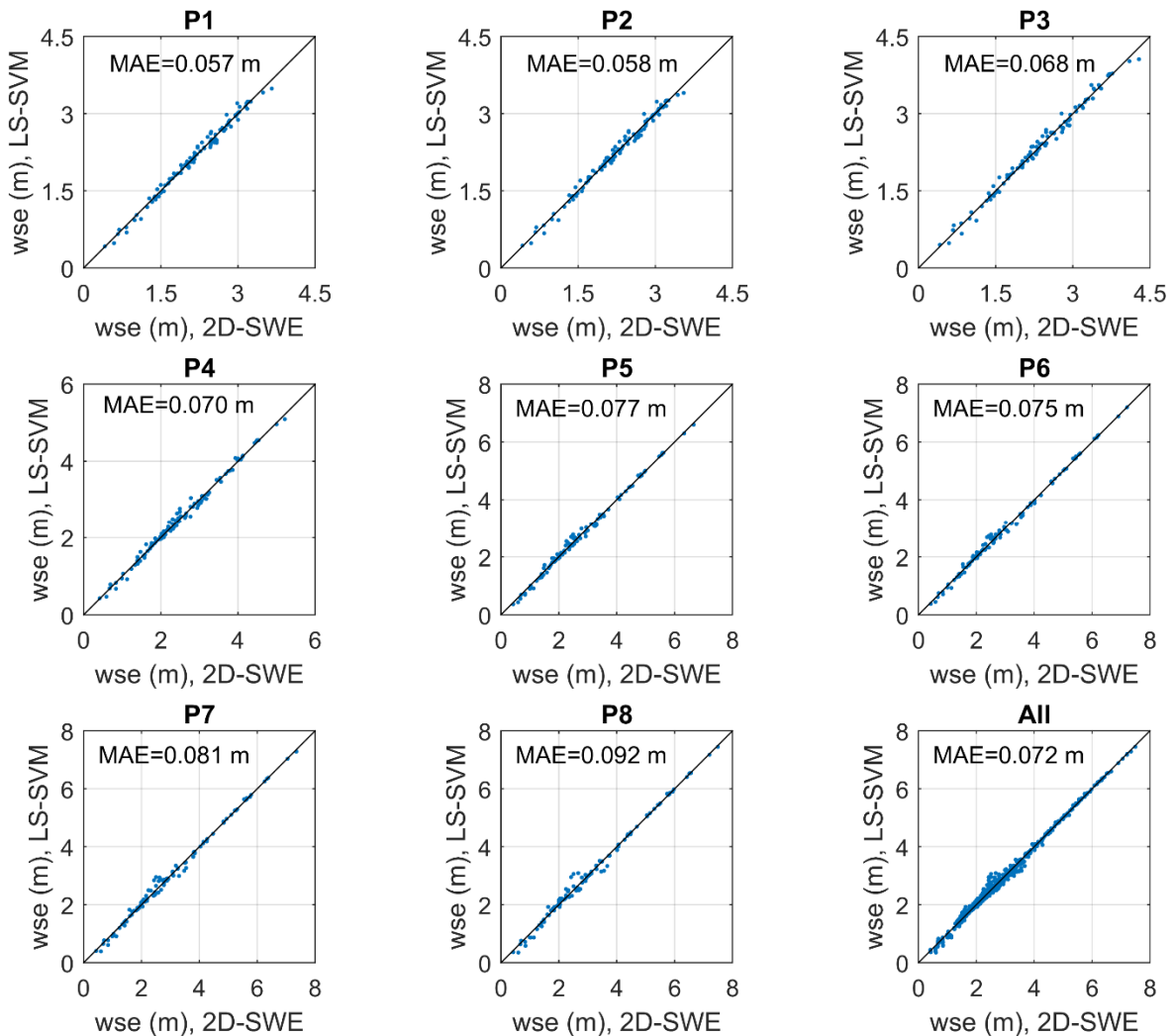
Figure 4. Scatter plot of water levels computed with the 2D-SWE model and the LS-SVM model in validation, with the 1:1 line plotted for reference in black. The mean absolute error in each point and the global mean absolute error, considering the 8 control points, for the 100 validation runs is indicated in the upper left-hand corner of the corresponding subfigure.
