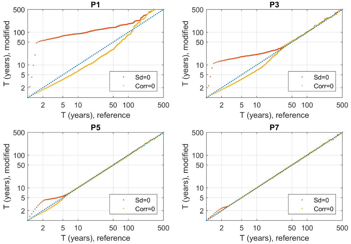
Figure 8. Changes in return period between the original simulation (x-axis) and the simulation that neglects the storm surge ( S_d=0 ), and the simulation that neglects the correlation between the storm surge and the river discharge ( Corr=0 ) (y-axis). The 1:1 line representing no changes in return period is plotted in blue.
