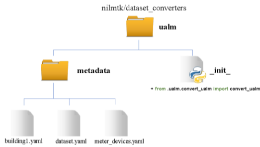
Fig. 4. Metadata file structure.
