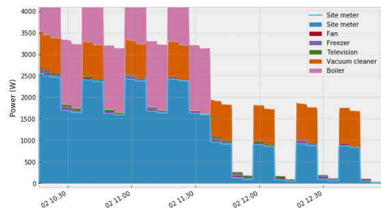
Fig. 7. Power profile.
