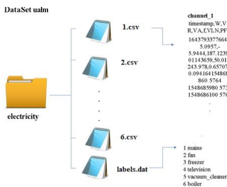
Fig. 5. Structure of data files.
