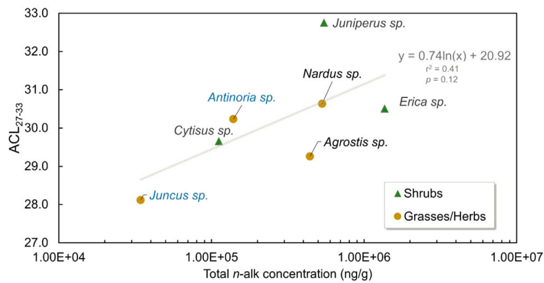
FIGURE 4 ACL_{27-33} vs. total n -alkane concentrations (ng/g, in logarithmic scale) of the two dominant ecological forms of the Lake Peixão catchment. The overall trend is represented by a logarithm regression line in gray. Green triangles represent shrubs; colored circles represent grasses/herbs, aquatic-related plants in blue, and nonaquatic plants in yellowish.
