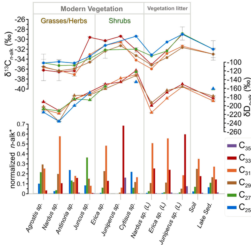
FIGURE 3 n -alkane distributions and compound-specific isotopic values ( C_{25} – C_{35} ) of the dominant plants, vegetation litter (L), soil and surface sediment samples of the Lake Peixão area. The whiskers correspond to 1 SD, where multiple measurements on the respective compound were performed. *Normalization against the total n -alkane concentration of each sample.
