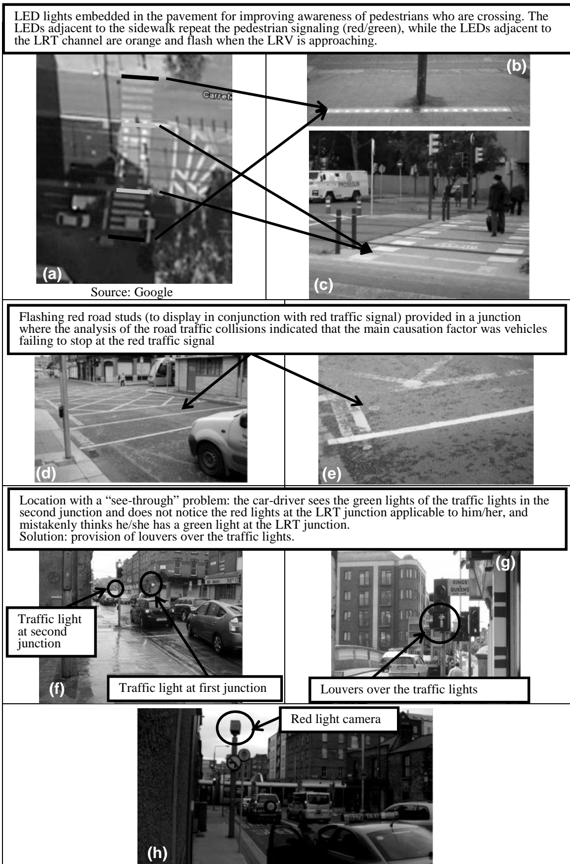
FIGURE 8 Innovative solutions at intersections. a,b&c) LED lights embedded in the pavement in Barcelona; d&e) Flashing red road studs in Dublin; f&g) “See-through” problem with louver solution in Dublin; h) Red light camera in Dublin.
