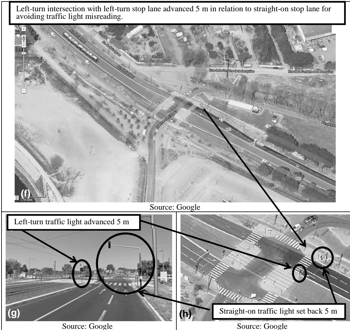
FIGURE 5 Left-turn intersections. a) Transforming a left-turn intersection into another kind of maneuver; b&c) Transforming a left-turn into a perpendicular intersection in Porto; d&e) Avoiding forbidden left-turns by means of bollards in Barcelona; f,g&h) Improving traffic lights readability in Montpellier.
