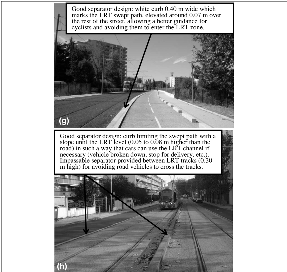
FIGURE 4 LRT separators on segregated channels. a) Parking forbidden along the separator in Tenerife; b,c,d&e) Green separators in Porto; f) Sidewalk-alike separator in Montpellier; g) Curb separator in Montpellier; h) Curb separator between both LRT directions in Montpellier.
