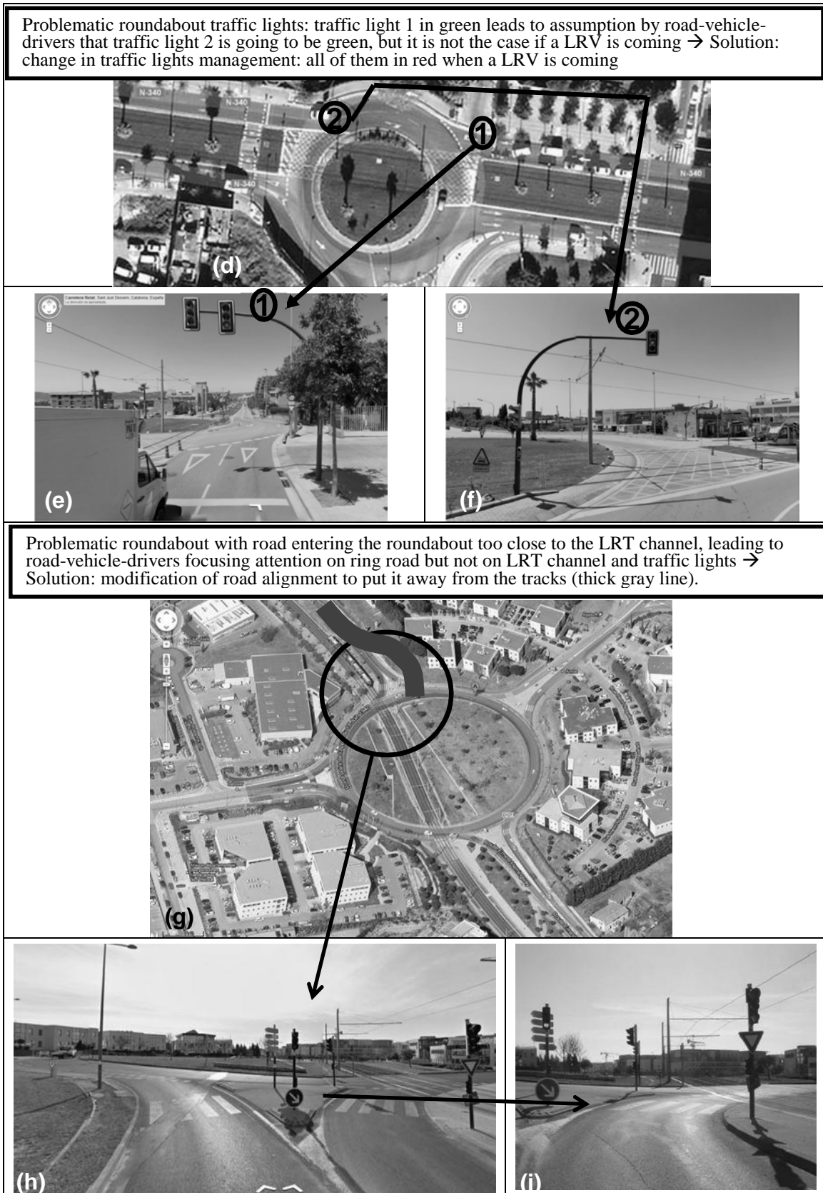
FIGURE 6 Roundabouts. a) Low vegetation in a LRT roundabout in Tenerife; b) Traffic lights for different approaching directions in Tenerife; c) Double small traffic lights for improving awareness in Tenerife; d,e&f) Modification of traffic lights operation for improving roundabout safety in Barcelona; g,h&i) Modification of the road layout for improving roundabout safety in Montpellier. Source: Google
