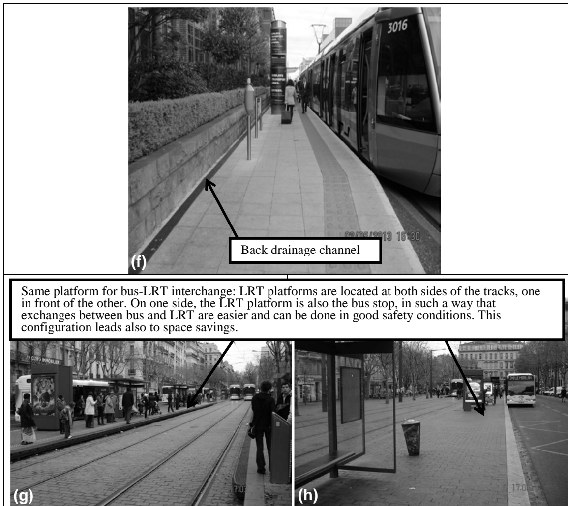
FIGURE 2 Platform design and station/stop location. a&b) Narrow platform without back barrier in Rome (Italy); c) Good platform design with back barrier in Dublin (Ireland); d) Excessive platform-vehicle gap in Rome; e) Narrow platform-vehicle gap in Tenerife (Spain); f) Back platform drainage channel in Dublin; g&h) Interchange between bus and LRT in the same platform in Marseille (France).
