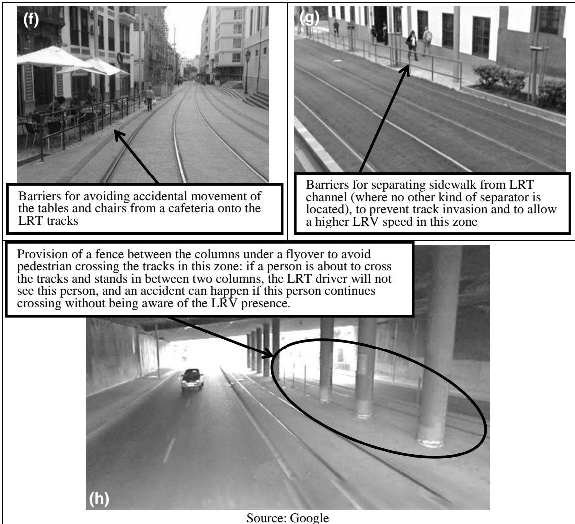
FIGURE 9 LRT channel differentiation and protection by means of pavement, marks, fences and barriers. a,b&c) Pavement treatment to avoid LRT tracks trespassing by road vehicle drivers in Dublin; d) Pavement treatment of a segregated channel in Dublin; e) Demarcation of swept path on shared channel in Dublin; f&g) Barriers for avoiding invasion in Tenerife; h) Fences for avoiding pedestrian crossing under a flyover in Tenerife.
