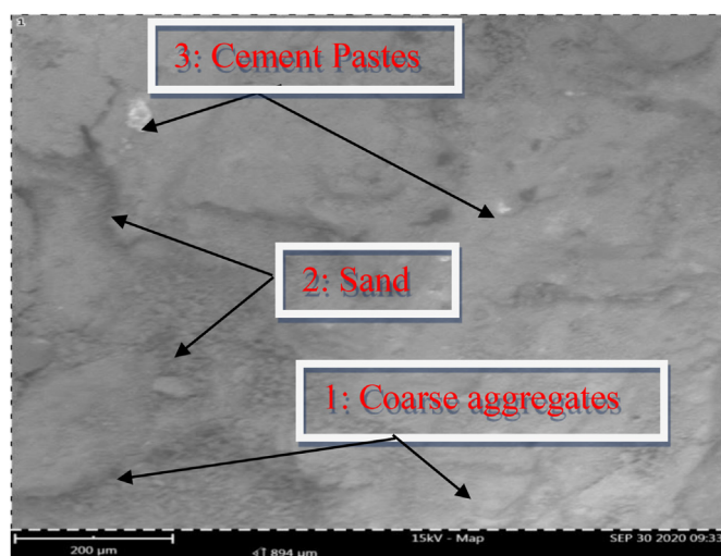
Figure 15. SEM micrograph of RHAC-10 HPC at 90 days.
