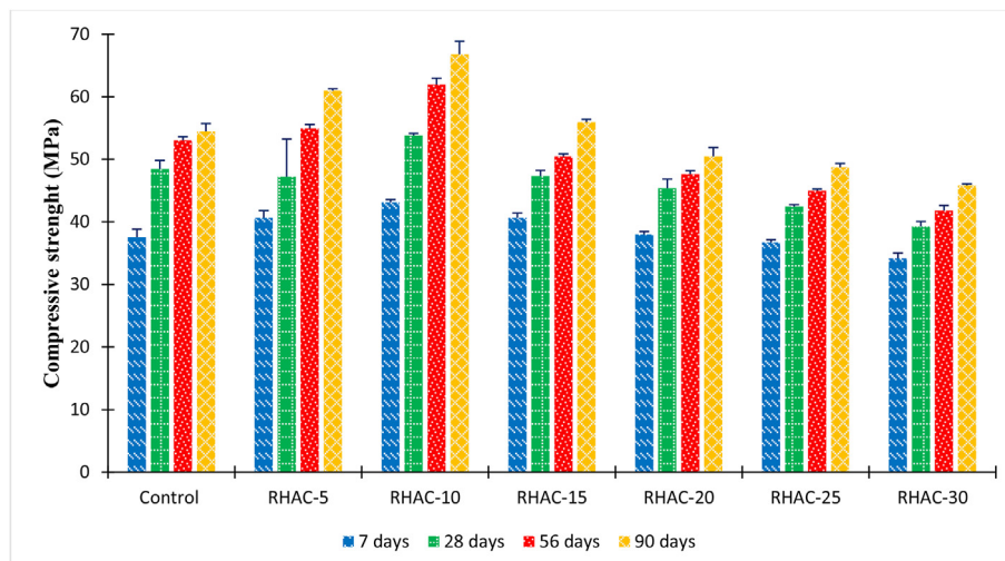
Figure 11. Compressive strength development of RHA-based HPC.
