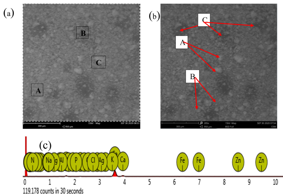
Figure 2. a–c: The SEM images and EDX patterns of CEM II (Nduka et al., 2022).
