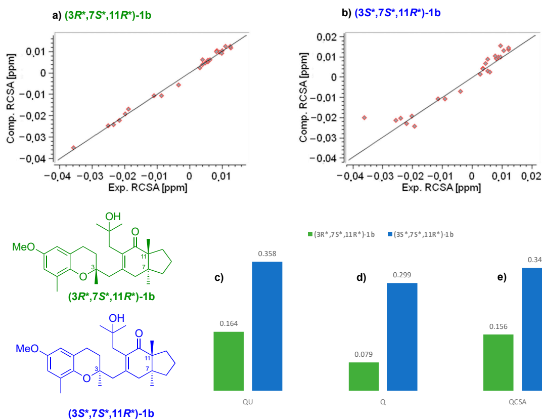
Figure 6. Anisotropic data ( 13 C-RCSA) of meroditerpene 1b swollen in 70/0.25 PMMA- d 8 gel (200 MHz, CD 2 Cl 2 ). (a,b) Fitting for carbon residual chemical shift anisotropies of diastereoisomers (3R*,7S*,11R*)- 1b (green) and (3S*,7S*,11R*)- 1b (blue), respectively. (c) Q U : quality factor of uncorrected RCSAs; (d) Q and (e) Q CSA quality factors for the configurations.
