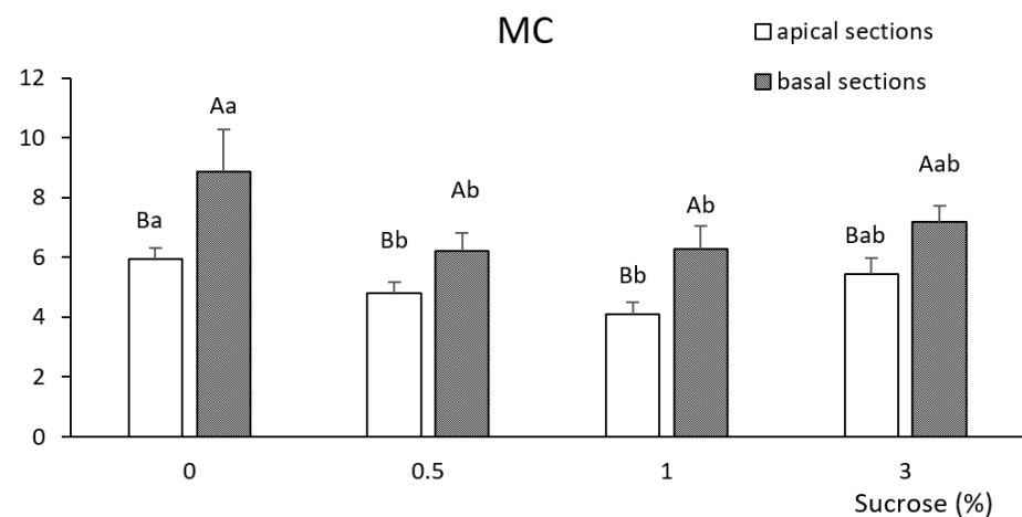
Figure 5. Effect of explant type and sucrose supplementation on multiplication coefficient of willow. Apical and basal sections were grown in RITA ® under 150 \mu\text{mol m}^{-2}\cdot\text{s}^{-1} PPF. For immersion in liquid medium, \text{CO}_2 -enriched air was applied for 1 min every 4 h. Values are the mean \pm standard error from 2 RITA ® vessels. Different capital letters indicate significant differences in relation to explant type, and different lowercase letters indicate significant differences in relation to the sucrose supplementation ( p < 0.05 ). MC—multiplication coefficient.
