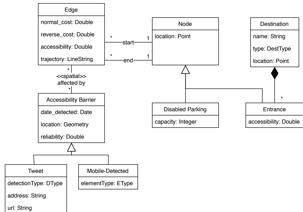
Figure 4. Data model.
