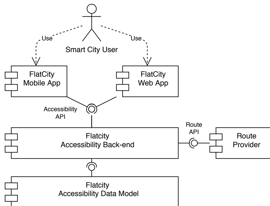
Figure 5. Application architecture.
