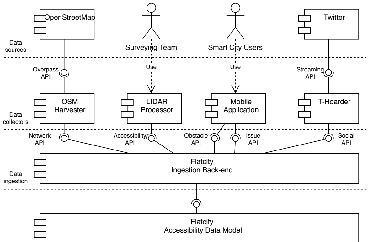
Figure 3. Ingestion architecture.
